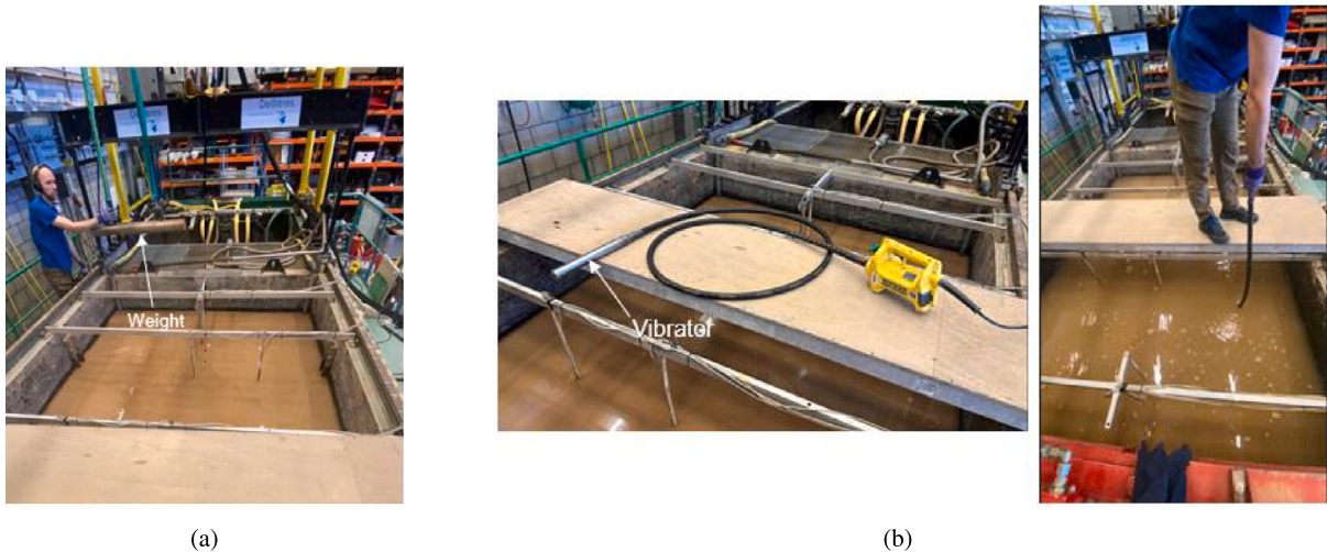
Fig. 8. Densification process in two steps: (a) densification with the use of a weight lifted by the crane and hitting the side walls of the container, and (b) densification of the sand bed by using vibrating needles.
