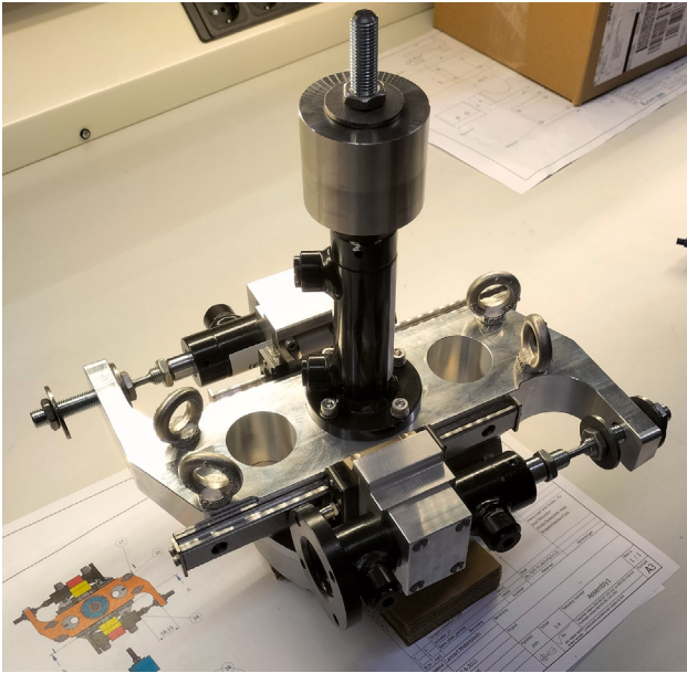
Fig. 2. The newly-developed lab-scale GDP shaker.
