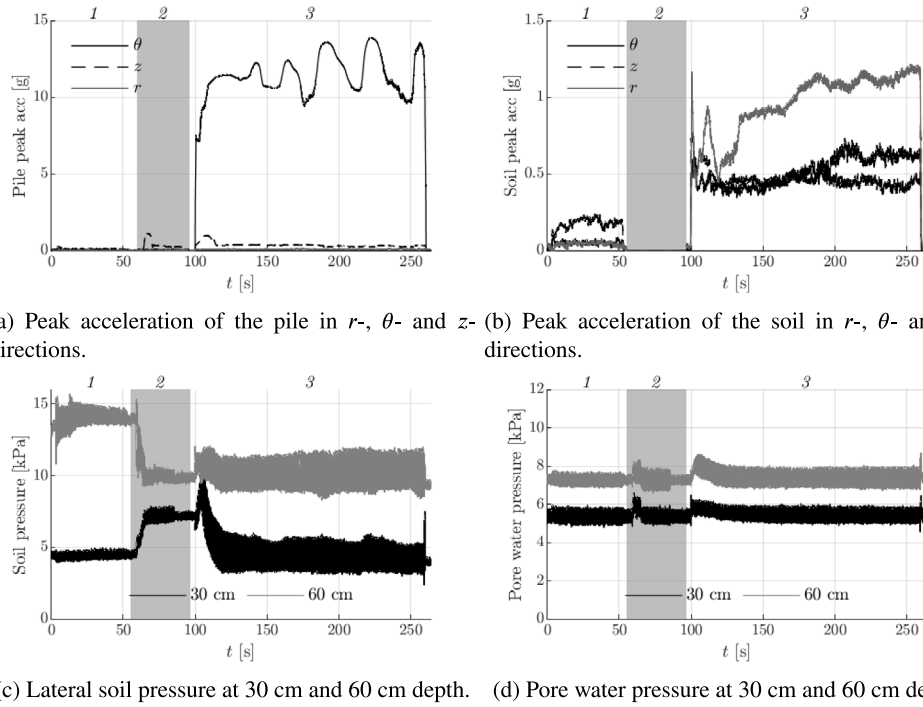
Fig. 15. Pile and soil response data as measured during tests in soil preparation 2.
