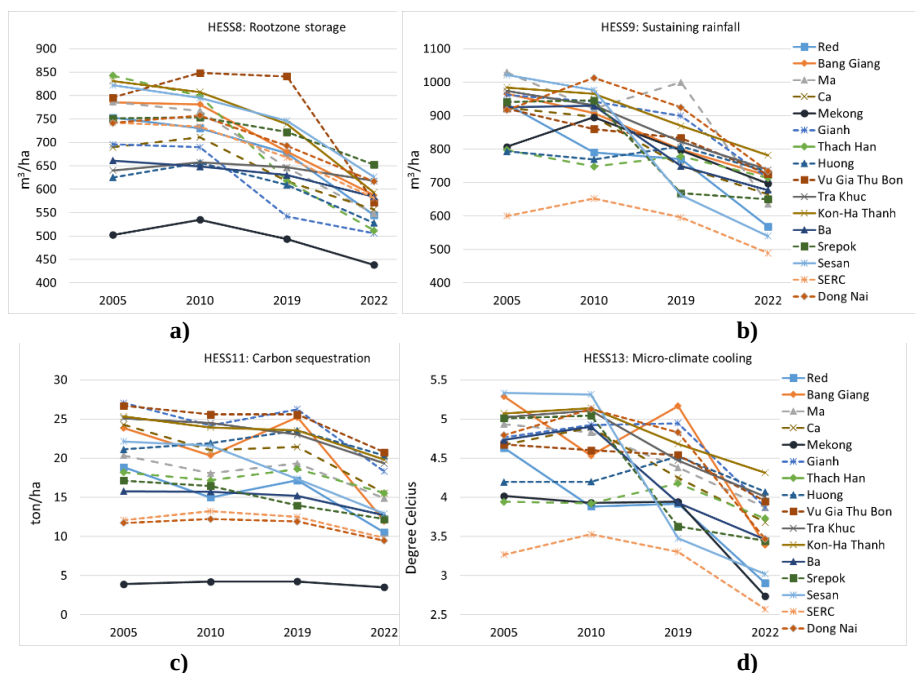
Figure 35. Trend of HESS that are declining a) HESS8: Rootzone storage; b) HESS9: Sustaining rainfall; c) HESS11: Carbon sequestration and d) HESS13: Micro-climate cooling
