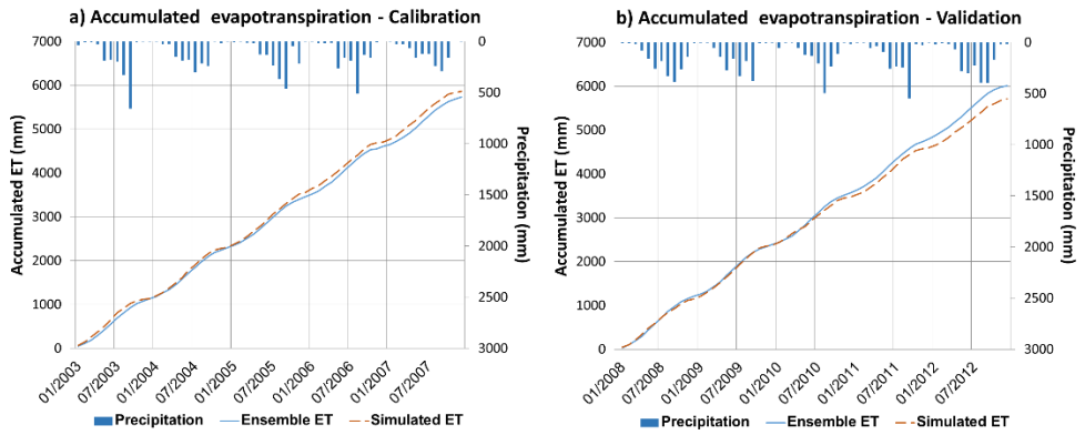
Figure 17. Accumulated ET for the period of five years for a) calibration and b) validation
