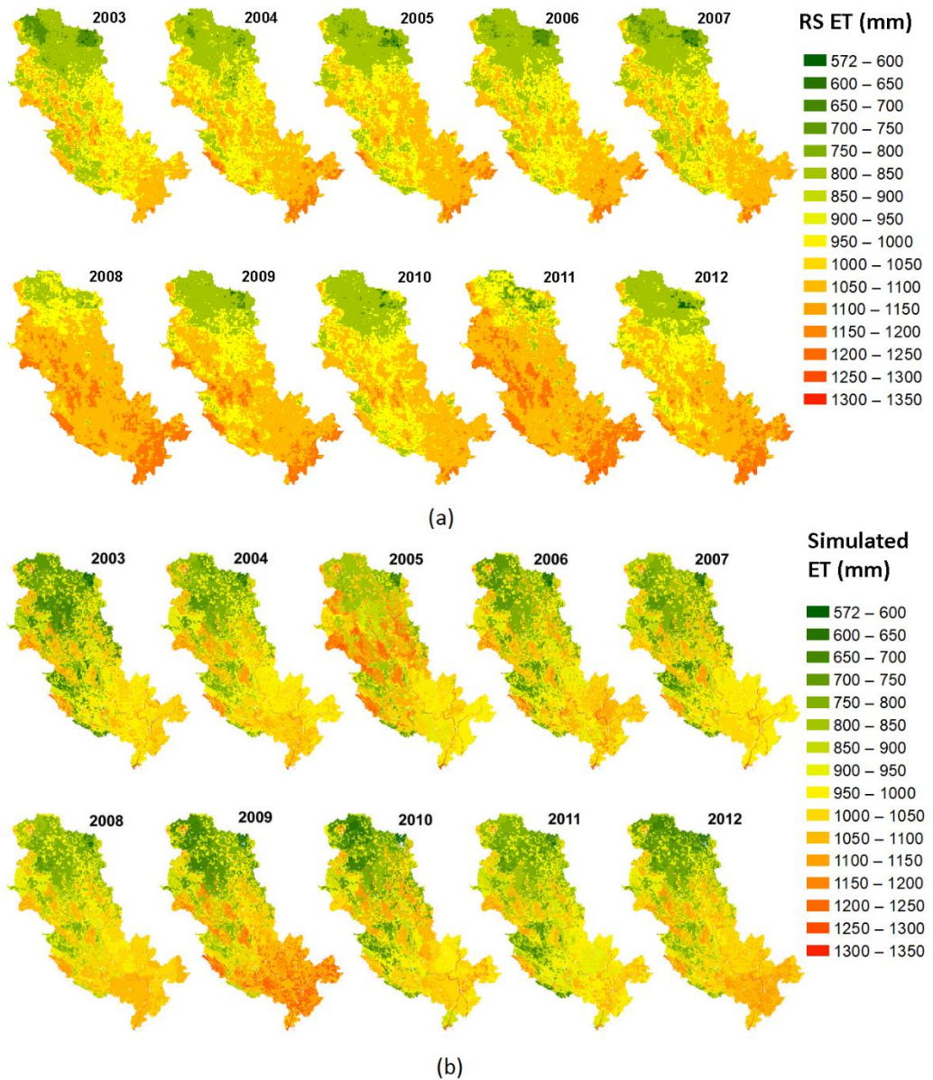
Figure 18. Spatial agreement between the ensemble ET from remote sensing (a) and the SWAT simulated ET (b) at an annual basis.
