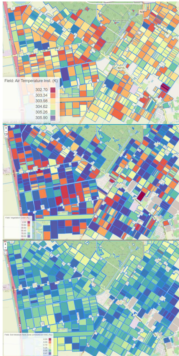
Figure 7. Example of midday air temperature on a field-by-field basis in the Noordoostpolder (The Netherlands) on 12/8/2020 based on actual vegetation cover and soil moisture conditions.
