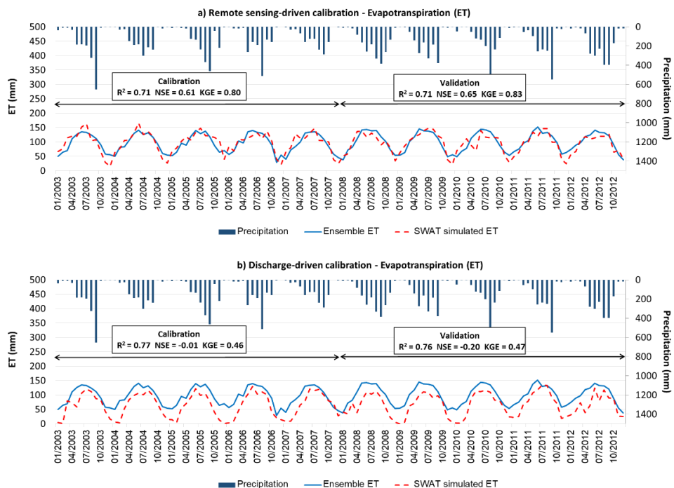
Figure 15. Temporal variability estimated from SWAT and the “observed” values from remote sensing in (a) remote sensing-driven calibration, and (b) conventional discharge-driven calibration.
