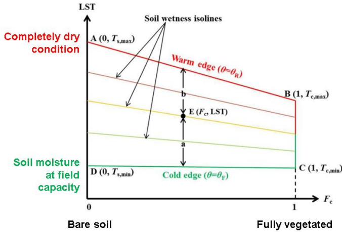
Figure 27. Trapezoidal method for estimating four extreme conditions (i.e., four corners) representing vegetation coverage/land surface temperature ( F_c/LST ) space (WaPOR database methodology, 2020; Yang et al., 2015)
