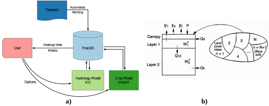
Figure 28. Schematization of a) RHEAS model [307] and b) the water balance component using VIC model [177]
