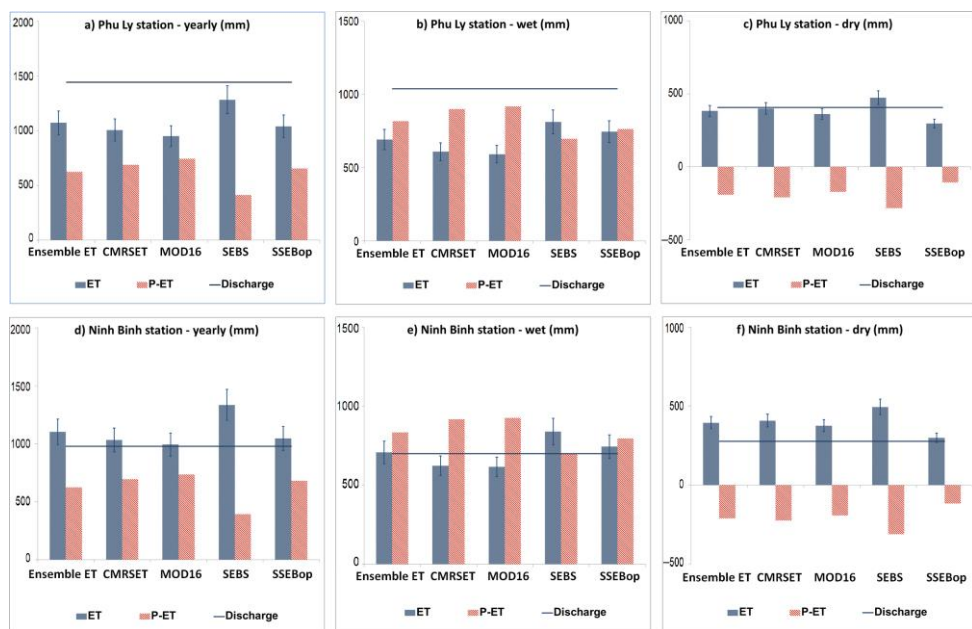
Figure 12. Comparison of accumulated evapotranspiration ( \Sigma ET ), rainfall surplus \Sigma P - \Sigma ET , and discharge \Sigma Q over the 2007 to 2010 period at yearly (a,d), wet months (b,e), and dry months (c,f) at two stations, Phu Ly and Ninh Binh.
