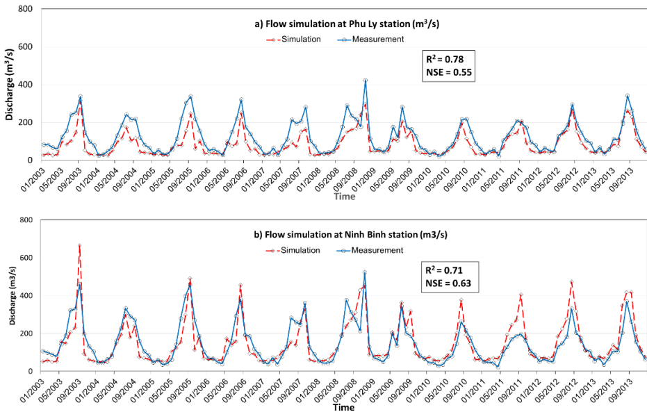
Figure 19. Flow simulation vs. station measurements at Phu Ly (a) and Ninh Binh station (b).
