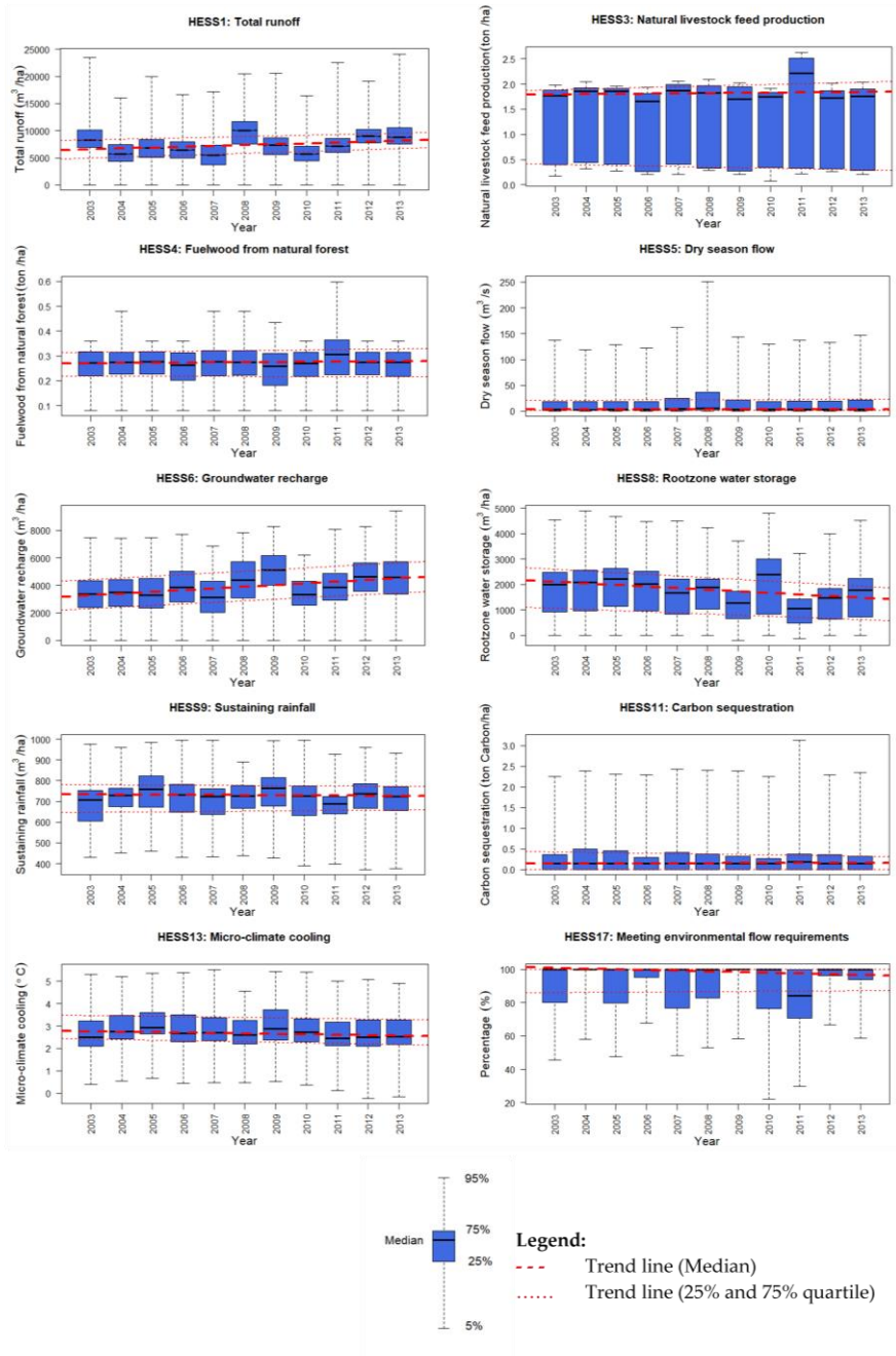
Figure 25. Boxplot values of ecosystem services for Day Basin from 2003–2013 and yearly average with median, quantile (5%, 95%), and quartile (25% and 75%). The dashed and dotted red lines show a trend line through the median, 25%, and 75% quartile, respectively.
