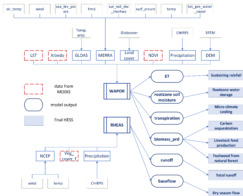
Figure 29. Hydrological Ecosystem Services (HESS) calculation routine with WaPOR and RHEAS model
