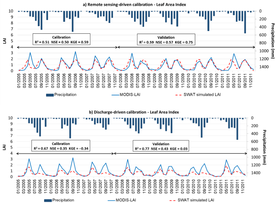
Figure 16. Determination of the LAI from MODIS and SWAT simulation for an HRU consisting of paddy rice for (a) remote sensing-driven calibration and (b) conventional discharge-driven calibration.
