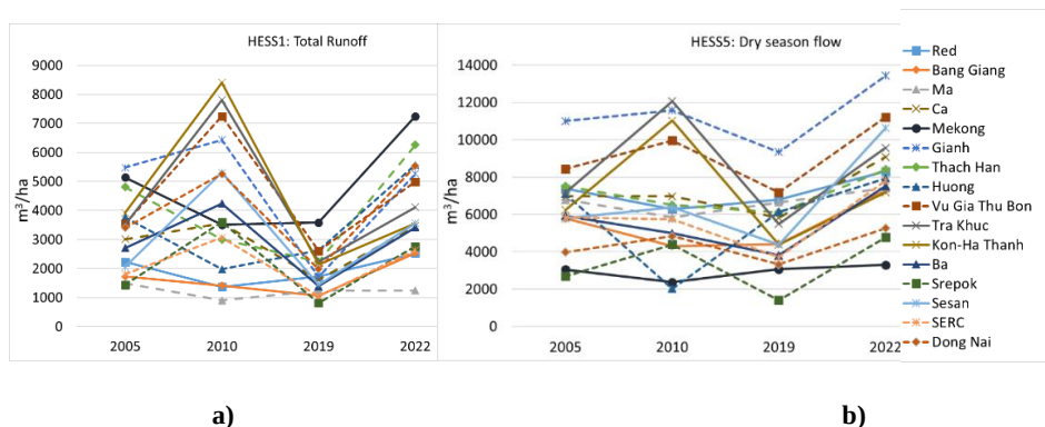
Figure 36. Trend of HESS that are increasing: a) HESS1: Total runoff; b) HESS5: Dry season flow
