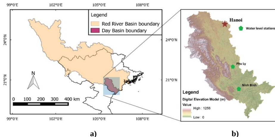
Figure 9. a) Geographical location of the Day Basin as part of the Red River delta in Northern Vietnam; b) Digital Elevation Model from Shuttle Radar Topography Mission (SRTM) for the Day River Basin and the location of two water level stations.
