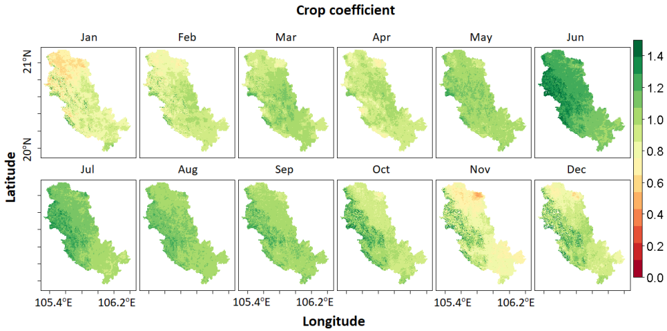
Figure 13. Monthly crop coefficient ( K_c ) derived from the ratio between the ensemble ET and reference ET.
