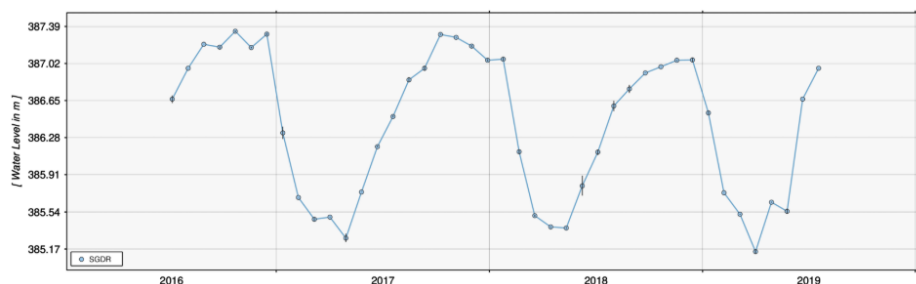
Figure 4. Changes in the water level of the White Nile near Kodok in South Sudan measured by the altimeter on Sentinel-3A. Base flow is pertinent when the water level is at approximately 385.4 m AMSL (source Dahiti, Technical University of Munich) ( http://dahiti.dgfi.tum.de/11745/ ) [109].
