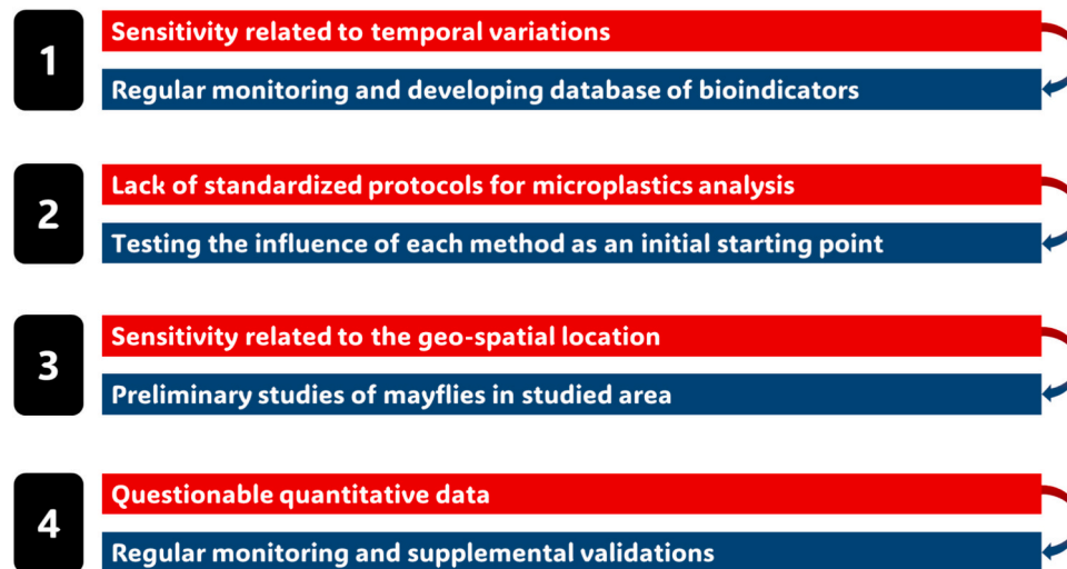
Fig. 3. Current challenges and suggested future approaches for the use of mayflies as bioindicator of heavy metals and microplastic pollutions.
