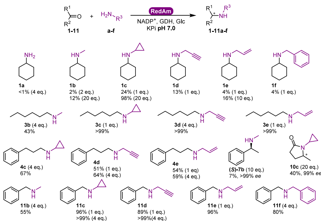
Figure 7. Reductive amination of carbonyl:amine combinations catalyzed by RytRedAm. Conditions: 100 mM KPi pH 7.0, 0.5 mg/mL RytRedAm, 30 mM Glc, 6 U/mL BsGDH E170K_Q252L, 10 mM carbonyl, 10–200 mM amine (equivalents of amine donor in parentheses), 0.2 mM NADP + , 500 rpm, 30 °C, 24 h. Average of duplicates. *: Absolute configuration not assigned, opposite to that obtained with AspRedAm.
