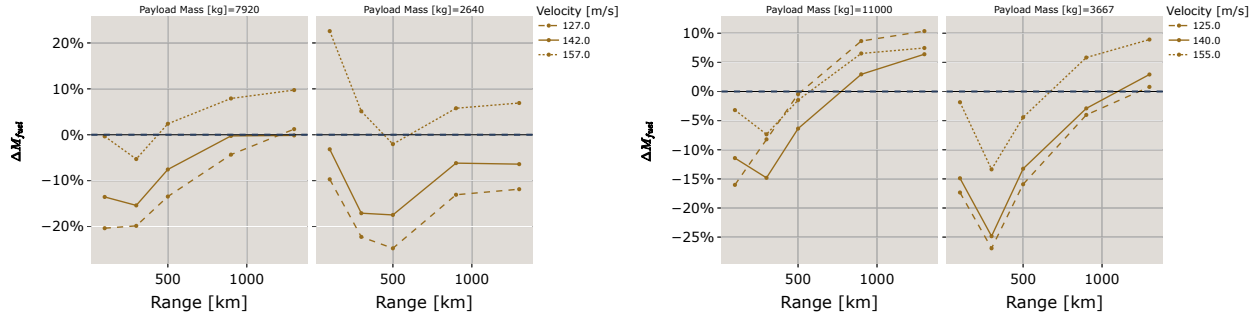
(a) Off-design analysis of ATR72-600HE aircraft (\phi = 5\%, R_{design} = 1370 \text{ km}, \text{Seats} = 72)
