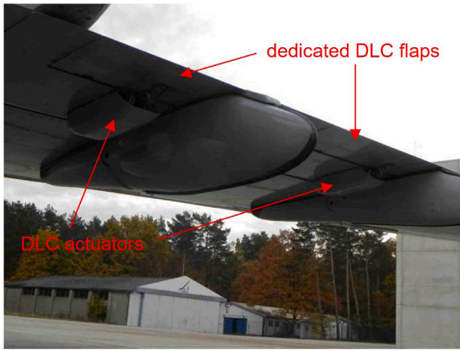
Fig. 6. DLC flaps at the trailing edge of the wing on ATTAS. Source: DLR.
