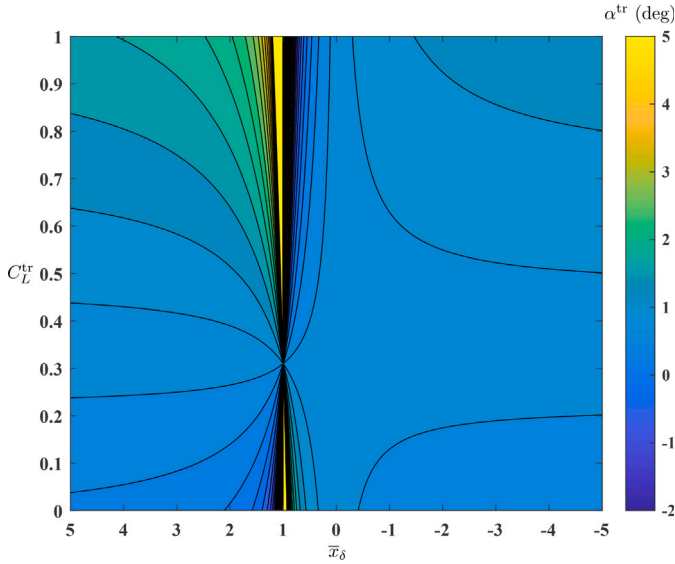
Fig. 14. Contour plot of \alpha^{tr} for different values of \bar{x}_\delta and C_L^{tr} , with C_{L_0} = 0.21 , C_{L_\alpha} = 0.119/\text{deg} , and \alpha_{\delta_{1,2}=0}^{tr} = 0.84 \text{ deg} .
