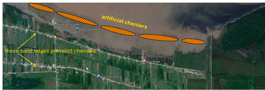
Fig. 10. Conceptual design artificial cheniers around Weg naar Zee (Suriname) to restart natural coastal dynamic processes.
