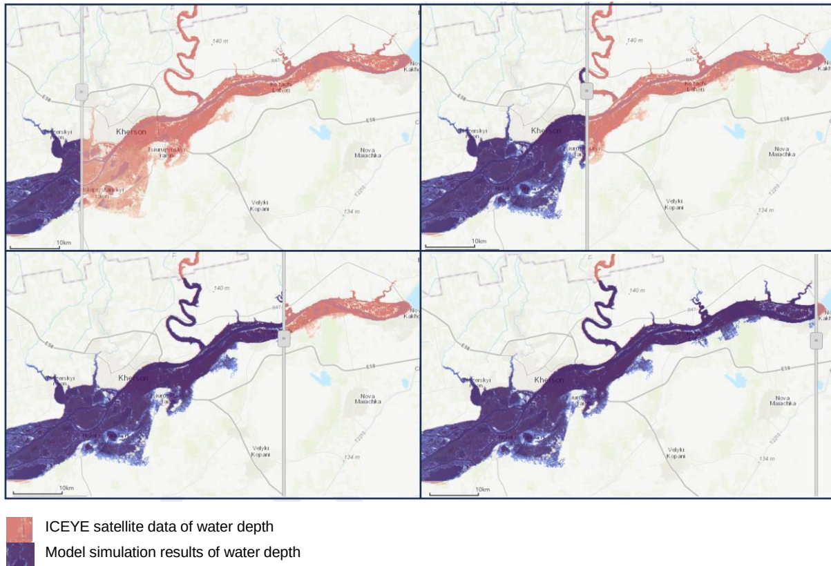
Figure 5: Comparison of modeled flood depths with ICEYE satellite results.
