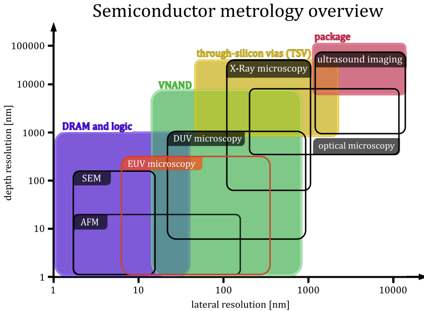
Figure 1.1: Semiconductor devices have a large range of lateral dimensions going from dynamic random-access memory (DRAM) and logic circuits [11, 12] with features in the nanometer regime, to microscopic non-volatile memory (VNAND) [13, 14], and to macroscopic semiconductor packaging [15, 16], each requiring different metrology needs. For larger-scale or high-speed applications, acoustical imaging and optical techniques such as microscopy, reflectometry, and scatterometry are typically employed. Tools like scanning or transmission electron microscopy (SEM, TEM) and atomic force microscopy (AFM) are often used at the nanoscale. Extreme UV (EUV) metrology, the main focus of this thesis, is projected to sit between these two regimes. Image reproduced from [17].
