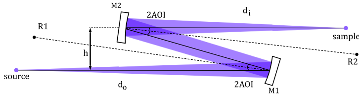
Figure 4.15: As mentioned before, spherical mirrors with a multi-layer coating could be used as well for illumination. A dual spherical mirror system was initially considered for the EUV beamline. The mirror set had a double function of imaging the source on the sample and to change the beam height h . This initial concept had a relatively small illumination NA of 0.0017, due to a small angle of incidence of 2.5 degrees in order to limit spherical aberration.
