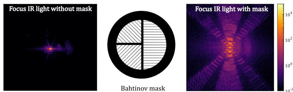
Figure 4.23: Without introducing any attenuation (or reduced repetition rate) of either the IR beam or EUV beam, capturing non-overexposed images of the beam near the focus becomes rather tricky. At a lower flux, non-overexposed images can be made without much detail due to the rather large pixels and a small probe when performing a through-focus scan. Placing a binary transmission Bahtinov mask, consisting of three sections with two diagonal gratings and one horizontal grating, as close as possible to the ellipsoidal mirror results in additional diffraction orders in the focal plane. The 0 th still closely represents the probe without a mask, but the energy is more dispersed across the camera, relieving the exposure problem. The main benefit of the mask is the ability to find the focal plane, as shown in Fig. 4.24. Note that the image on the right is on a log scale.
