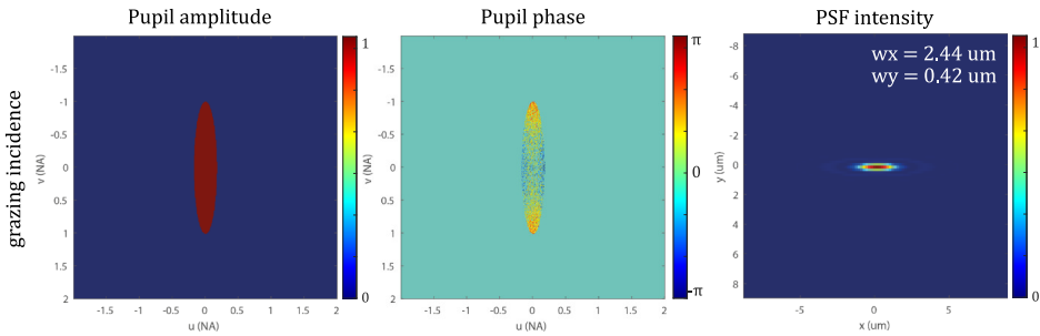
Figure 4.18: The designed ellipsoidal mirror with parameters a = 705 mm and b=c= 77.66 mm is illuminated at a grazing incidence angle of 10 degrees. A ray-traced probe of 0.42 by 2.44 \mu\text{m} is formed in the focus of the ellipsoid.
