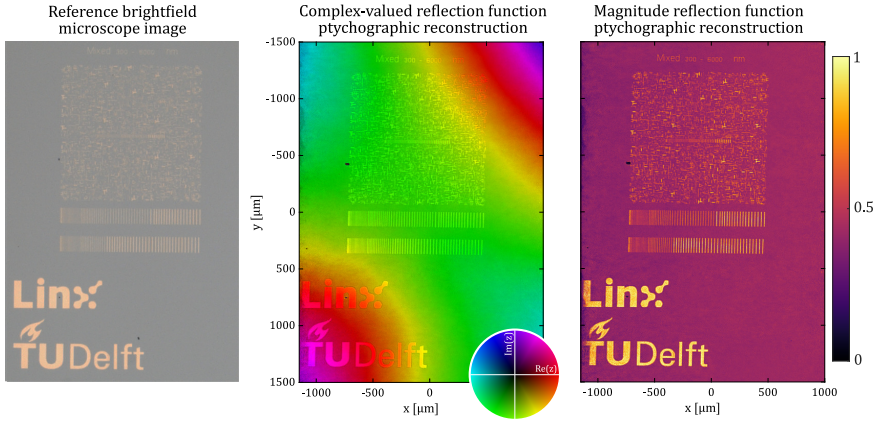
Figure D.5: Mixed 'Manhattan'-like structures, a chirped grating and the logo of LINX and the TU Delft are patterned on top of a silicon wafer. A ptychography scan has been performed in reflection at 45 degrees angle of incidence using light with a wavelength of 660 nanometer. The reconstruction compares well to the conventional brightfield microscope image on the left.
