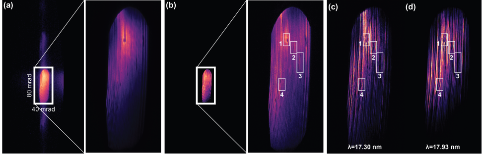
Figure 5.6: EUV focusing optics characterisation. (A): Summed intensity distributions of the diffraction patterns in logarithmic scale with zeroth order in the shape of the ellipsoidal focusing mirror and higher orders cropped in the horizontal direction due to the sample tilt in reflection geometry. Inset: zoom-in of the zeroth order in linear scale. (B): Reconstructed common background intensity in logarithmic with a clearly distinct ellipsoidal shape representing the pupil of the illumination system. Inset: zoom-in of pupil in linear scale. (C and D): Reconstructed pupil function of the illumination probe at wavelengths 17.30 nm (C) and 17.93 nm (D). The rectangular ROI 1-4 show the locations of the defects on the EUV focusing mirror.
