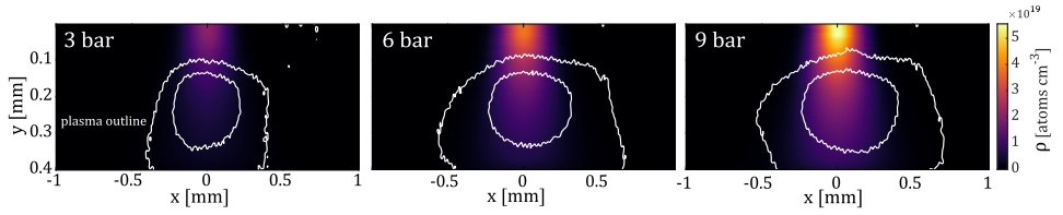
Figure 7.7: Reconstructed density profiles in atoms per cm 3 of an argon gas jet with a backing pressure of 3, 6 and 9 bar. For reference purposes, using the ideal gas law, 1 bar argon at room temperature has a density of 2.47 \cdot 10^{19} atoms per cm 3 . The white outlines represents the size of the observed plasma at a given backing pressure when the gas jet is exposed to the fundamental drive laser 2 . The center white line represents the half of the observed peak plasma brightness (FWHM) and the second line refers to the 1/e^2 value of the peak brightness.
