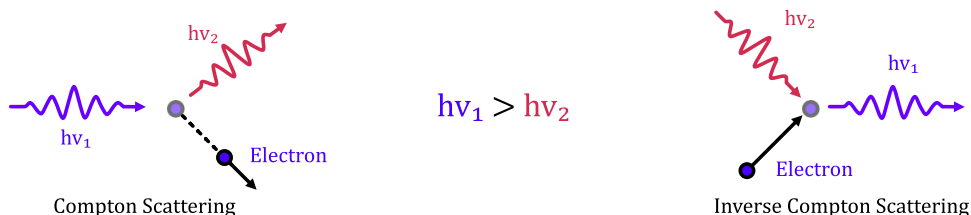
Figure 3.9: When a high-energetic photon collides with an electron it can scatter through Compton Scattering, transferring a part of the energy to the electron, resulting in a lower energetic photon. For Inverse Compton Scattering an energetic electron and a relatively low energetic photon collide resulting in a higher energetic photon, potentially in the X-Ray part of the spectrum.
