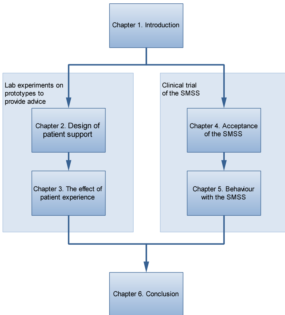
Figure 1.1: Thesis Outline
