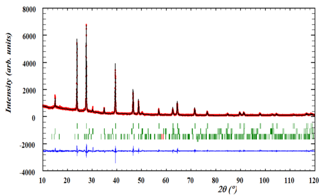
Figure 14. Profile refinement of the XRD obtained from the post-DSC sample at x(\text{MgCl}_2) = 0.3 in the \text{NaI-MgCl}_2 system. Phases used in the refinement are \text{MgCl}_2 , \text{NaI} and \text{Na}_3\text{Mg}_2\text{Cl}_8 . The observed intensity (red circles) is shown alongside the calculated intensity (black line), and the difference between the two is shown (blue line). The angles at which reflections occur, i.e., the bragg positions, are shown as well (green, vertical lines).
