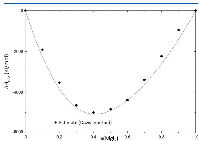
Figure 5. Mixing enthalpy of the NaI–MgI 2 system, calculated at T = 1000 K, compared to the estimated mixing enthalpy obtained using the estimation method of Davis and Rice. 8
