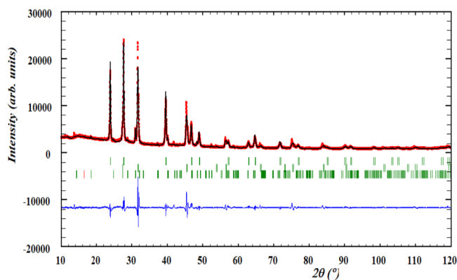
Figure 12. Profile refinement of the XRD obtained from the post-DSC sample at x(\text{MgI}_2) = 0.1 in the \text{NaI-MgI}_2 system. Phases used in the refinement are \text{NaCl} , \text{NaI} , \text{NaMgCl}_3 , and \text{Na}_6\text{MgCl}_8 . The observed intensity (red circles) is shown alongside the calculated intensity (black line), and the difference between the two is shown (blue line). The angles at which reflections occur, i.e., the bragg positions, are shown as well (green, vertical lines).
