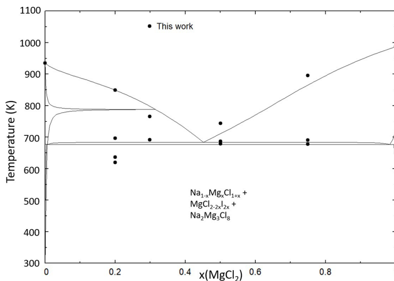
Figure 13. Phase diagram of the system \text{NaI-MgCl}_2 calculated with the optimized quaternary model presented in this work. Experimental data obtained in this work (black circles). The labeled phase field corresponds to the phase field where post-DSC XRD measurements have been performed.
