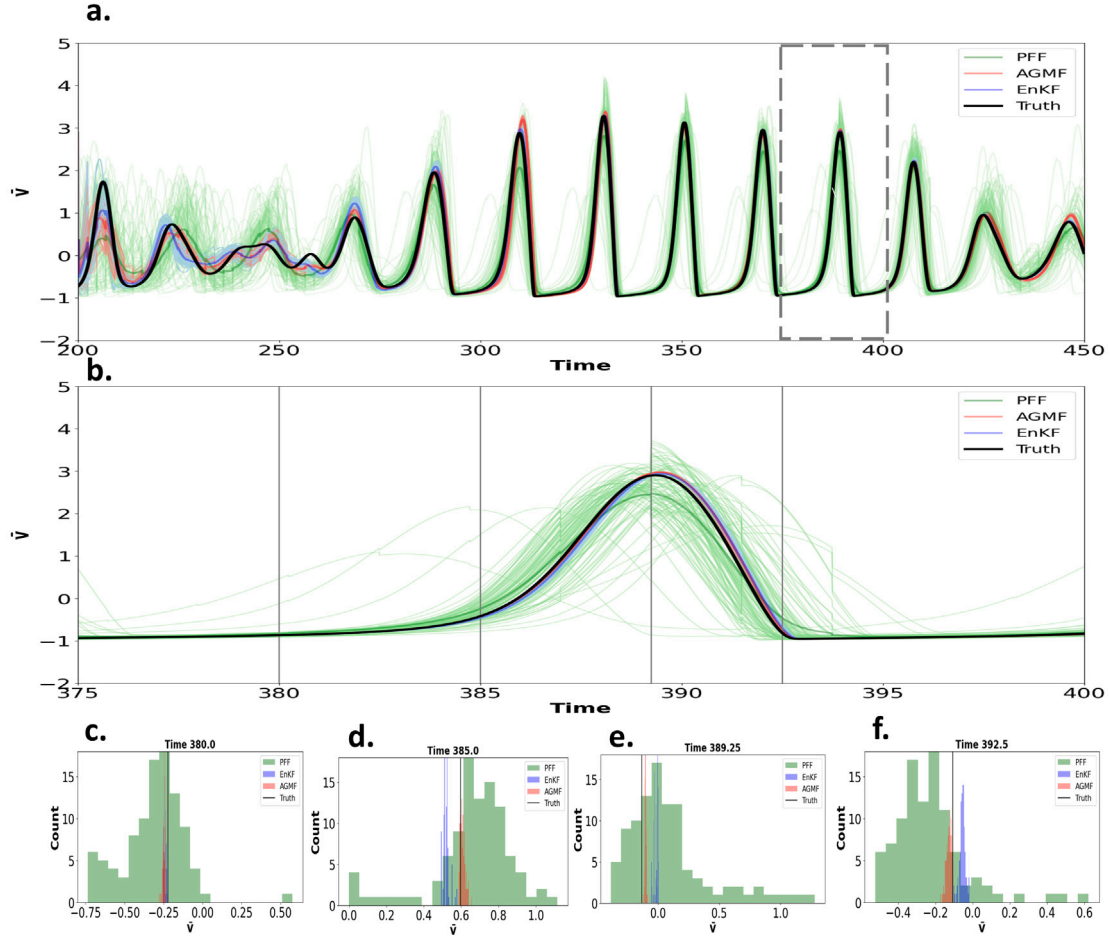
Fig. 8. Comparison of the estimates of the slip-rate ( \bar{v} ) of block 10 for the EnKF (blue), the AGMF (red), and the PFF (green) for estimating an earthquake occurrence for a chaotic event. The true time series of the slip-rate is shown with a solid black line. We compare the ensemble distribution for the interseismic phase (c,d) during the coseismic phase (e), and at the end of the coseismic phase (f).
