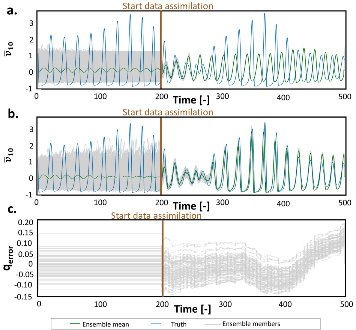
Fig. 10. Comparison of the estimates of the slip-rate \bar{v} at the block 10 of an EnKF (a) without model error and (b) with model error as part of the state vector. The mean values are in green. The truth, in blue, corresponds to the slip-rate of the chaotic model with \epsilon = 0.5 . The individual ensemble members in gray are periodic with \epsilon = 0.3 and model error. The synthetic observations are extracted from the chaotic synthetic truth. The results show that despite the parameter bias the EnKF estimates are in sync with the truth when including the model error especially in the occurrences of the seismic events, but with differences in the magnitude (amplitude of the signal). (c) Time series estimation of the q_{error} .
