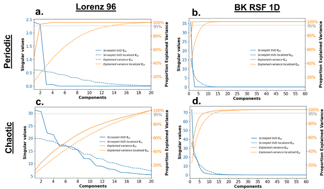
Fig. 14. Scree plot of the singular value decomposition of the prior covariance matrices ( C_{zz}^f ) before and after localization for the Lorenz 96 (a, c) and Burrige–Knopoff model (b, d). The solid lines correspond to the decomposition of the matrices before localization, while the dashed lines to the decomposition of the matrices after the localization. The blue lines represent the distribution of singular values while the orange lines show the proportion of cumulative variance explained until that component.
