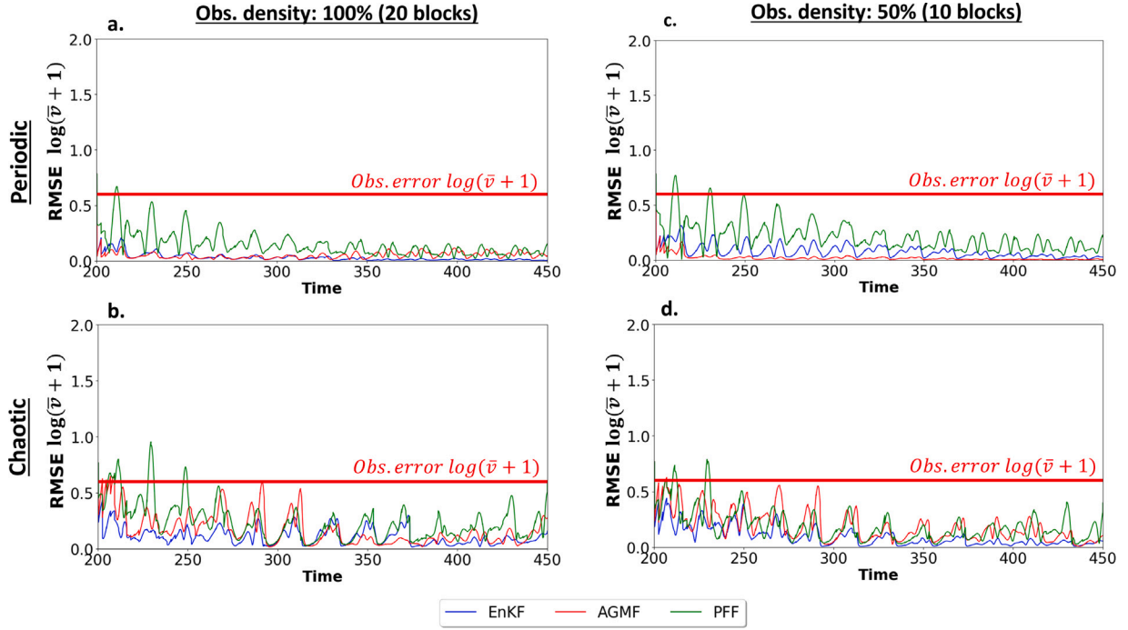
Fig. 4. Comparison of the RMSEs for the estimates of the logarithm of the velocity ( \log(\bar{v} + 1) ) of the EnKF (blue), the AGMF (red) and the PFF (green) for the 1-D Burridge Knopoff model coupled with rate-and-state friction. The upper row shows the comparison for the periodic case (a, c), and the lower row for the chaotic case (b, d). The results correspond to an observation density of 100% of the blocks for the left column (a, b) and 50% of the blocks in the right column (c, d).
