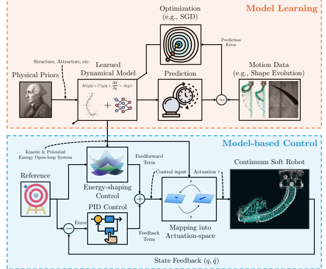
Fig. 1: Scheme of the main contribution - Model-based control of soft robots with learned models that exhibit a physical structure.
