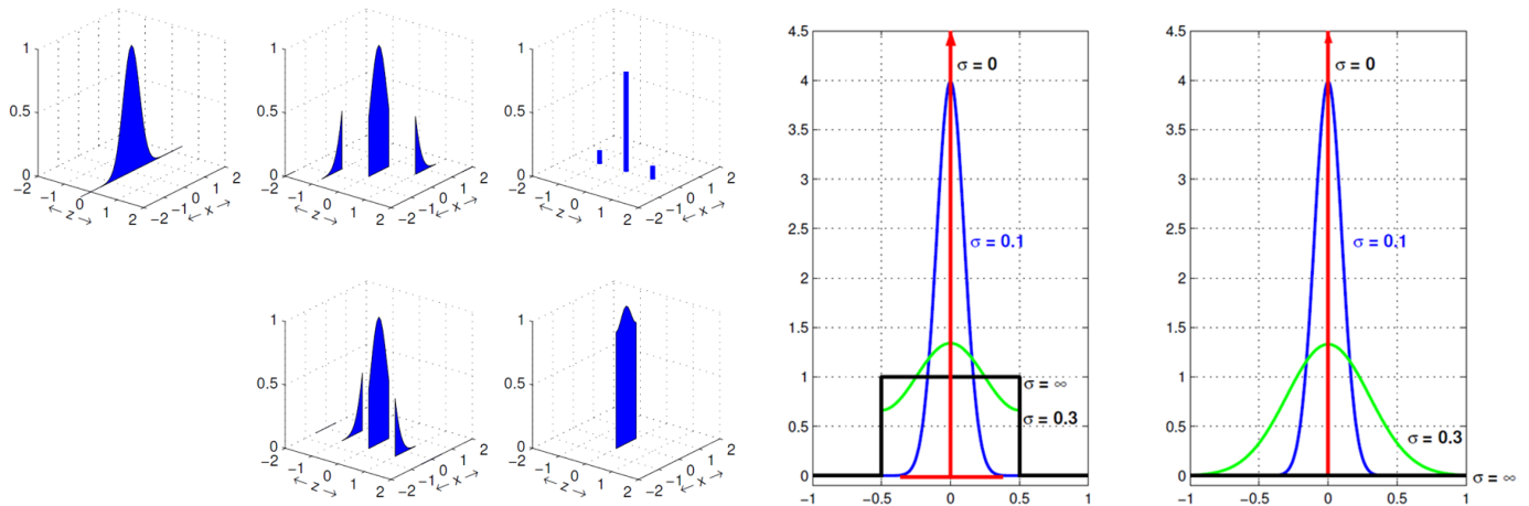
Figure 2. PDF ambiguity residual: (Left) Stepwise construction (in blue) of f_{\xi_0}(x) from f_{a_0}(x) (cf. (15)); (Right) PDF comparison between f_{\xi_0}(x) (left) and f_{a_0}(x) (right) for four different values of the standard deviation \sigma .
