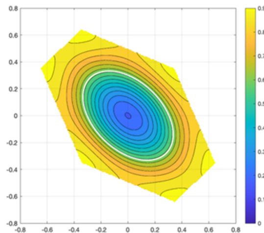
Figure 5. Contour plot with color bar of the integer testing power function F(\delta) = P[\|\hat{a}_0 - \check{\hat{a}}_0\|_{Q_{\hat{a}_0\hat{a}_0}}^2 > \tau_\alpha | \mathcal{H}_a] ( \alpha = 0.05 ) for a single-epoch, dual-frequency, GNSS geometry-free model. The horizontal and vertical axes are expressed in cycles.
