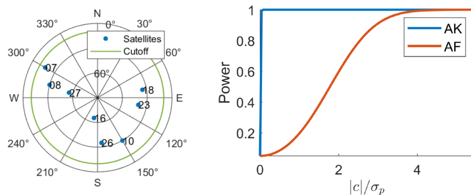
Figure 1. Tropospheric AK and AF power function curves, computed using their noncentral Chi-square CDF. Left: single-epoch GPS skyplot; Right: single-epoch, L1 GPS, \alpha = 0.05 , ambiguity-float (AF) and ambiguity-known (AK) power function curves for tropospheric zenith delay testing.
