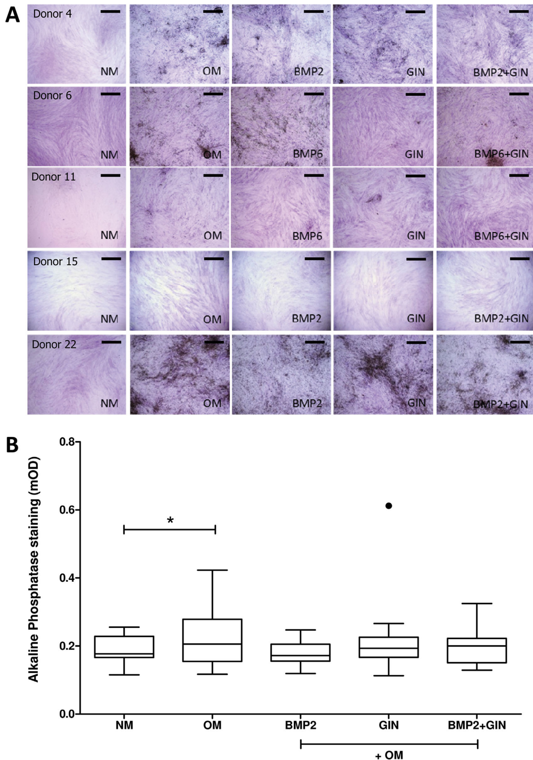
Figure 1. Alkaline Phosphatase (ALP) staining. (A) Pictures of ALP staining of cell cultures of five representative donors cultured in NM or stimulated with OM or OM supplemented with either BMP-2 or BMP-6, GIN and BMP-2 or BMP-6 + GIN. Bars represent 1 mm. (B) Boxplot showing the mOD after extraction of ALP staining from the cultures of twenty-two donors cultured in NM, OM or OM supplemented with either BMP-2, GIN or BMP-2 + GIN. Values represent mean \pm SD, dots represents 1.5 \times IQR. NM: normal medium; OM: osteogenic medium; BMP: bone morphogenetic protein; GIN: GSK3 \beta inhibitor; IQR: Inter Quartile Range. * p < 0.05 compared to NM.
