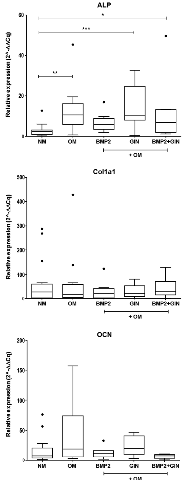
Figure 3. Relative gene expression ( 2^{-\Delta\Delta Cq} ) of cells stimulated with osteogenic stimuli. Expression of alkaline phosphatase (ALP), alpha-1 type I collagen (Colla1) and osteocalcin (OCN) was corrected for internal control GAPDH and the geometric mean of calibrators SaOS-2 and HDFA. Boxplot showing the mean \pm SD, dots represent 1.5 \times IQR. NM: normal medium; OM: osteogenic medium; BMP: bone morphogenetic protein; GIN: GSK3 \beta inhibitor; IQR: Inter Quartile Range. * p < 0.05 , ** p < 0.01 , *** p < 0.001 .
