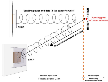
Figure 12: RFID communication system: this experiment use passive tag, which contains no battery, the tag-reader communication process is always initiated by the reader emitting antenna (RHCP), the tag can modulate the signal before transmitting it back to the receiver antenna (LHCP).
