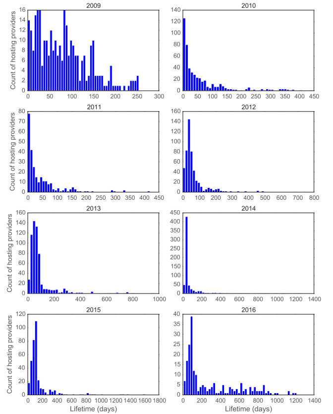
Figure 7: Distribution of C&C average uptime hosted by providers over years
