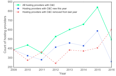
Figure 3: Time-series plot of providers hosting C&Cs
