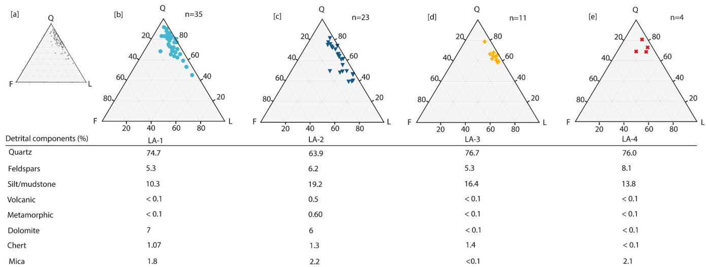
Fig. 8. Detrital composition data of the sandy lithofacies associations. a) All thin section data. b) Detrital composition data of stacked stratified sandstone (LA-1). c) Detrital composition data of fining-upward sandstone (LA-2). d) Detrital composition data for coarsening-upward sandstone (LA-3). e) Detrital composition data for thin-bedded sandstone (LA-4).
