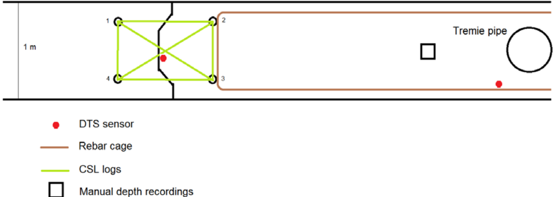
Figure 19: Position of CSL logs, manual depth recordings and DTS sensors in the panel
