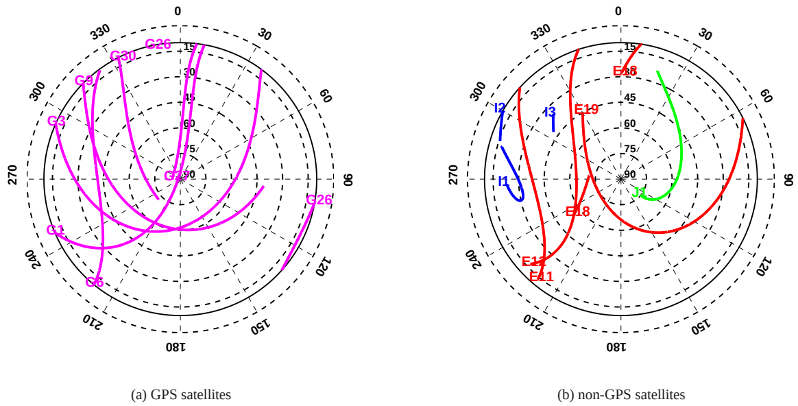
Figure 2. Experiment I: skyplot of GPS BLOCK II-F (magenta), Galileo (red), QZSS (green) and IRNSS (blue) satellites with L5/E5a-signal in Perth, Australia during the period considered (Table 2), with 10^\circ elevation cutoff
