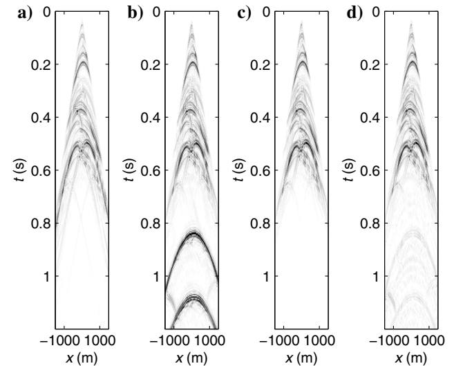
Figure 5. (a) Reflection response from below with a source at \mathbf{x} = 0 on \partial\mathcal{V}_j and receivers on the same level, computed in the reference medium. A similar reflection response, retrieved by single-sided redatuming of focusing functions (i.e., inversion of equation 23). Similar reflection responses, retrieved by target-enclosed redatuming of the (c) Green's functions (i.e., inversion of equation 15) and (d) focusing functions (i.e., inversion of equation 24). All figure parts have been normalized with respect to their maximum value.
