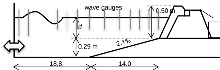
Figure 2. Model setup in LNEC flume.
