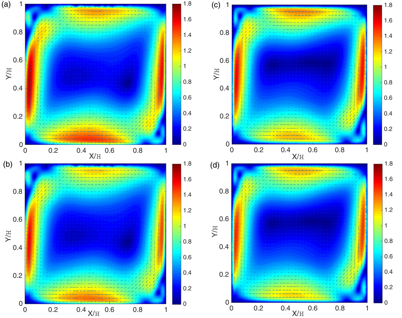
FIG. 3. Mean velocities ( |\bar{u}| ) contour plots in a vertical cross section at half-depth of the cell ( Z/H = 0.5 ). Velocity values normalized by U_{LSC(GL)} in panels (a) and (c) and by U_{LSC(P)} in panels (b) and (d). Panels (a) and (b) Non-Boussinesq: Ra = 6.91 \times 10^8 , Pr = 4.33 ; panels (c) and (d) Boussinesq: Ra = 6.74 \times 10^8 , Pr = 7.24 .
