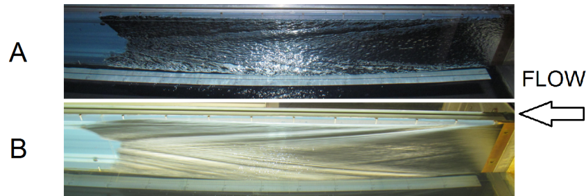
Figure 4 – Different wavesystems on the external cavity surface, V=1.5 m/s. A: instantaneous wave profile. B: time averaged wave profile (reproduced from [2]).
