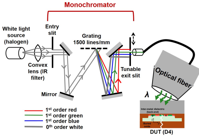
Fig. 20. Schematic of the experimental set-up used to measure the transmission spectrum of the inter-metal dielectric stack covering the SJ-LEDs. The SJ-LED is operated as a photo-diode by illuminating it with light at finely resolved wavelengths ( \approx 5 nm). The measured short-circuit current
