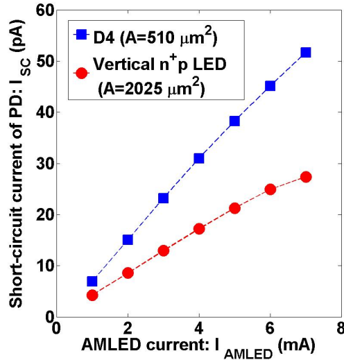
Fig. 18. Comparison of the PD short-circuit current when illuminated by the SJ-LED D4 (blue) and a conventional n^+p AMLED (red) in the same technology with a V_{\text{BR}} of 16.8 V, showing a \approx 2 times higher IQE for D4 at a given I_{\text{AMLED}}=4 mA.
