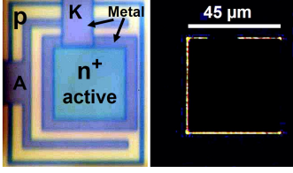
Fig. 17. Top-view (left) and the AM-EL micrograph (right) of the conventional n^+p AMLED at I_{\text{AMLED}}=4 mA. The field and hence EL dominated over the perimeter of the n^+ active area.
