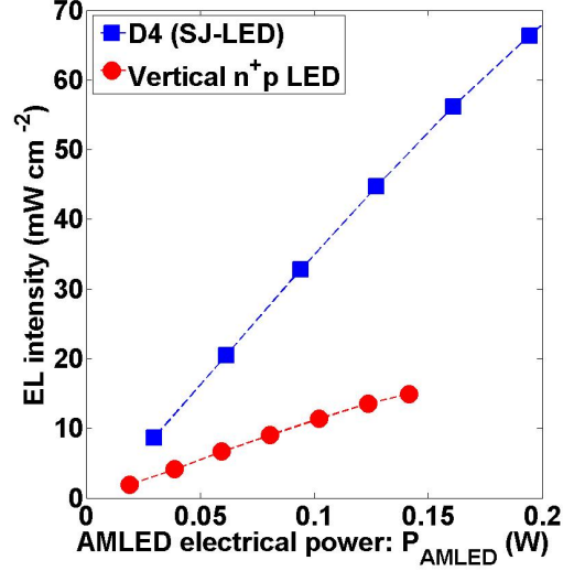
Fig. 19. Comparison of the AM-EL intensity along y-axis of the SJ-LED D4 (blue) and the conventional n^+p AMLED (red) versus P_{\text{AMLED}} . For the same P_{\text{AMLED}} , the EL-intensity of D4 is \approx 3 times higher than that of the conventional AMLED.
