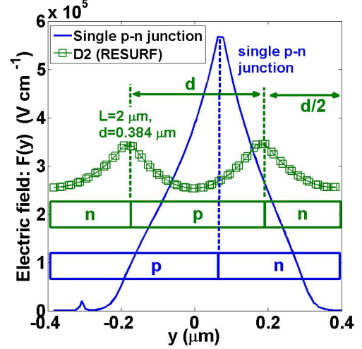
Fig. 6. TCAD simulated field profiles F(y) at V=52 V for D2 (green), showing its hyperbolic shape and more uniformity as compared to a single p-n junction (blue) of a similar size (as a guide to the eye) at a suitable V . Pinch-off of the depletion regions in the fingers (eq. (2)) occurs at V < V_{\text{BR}} .
