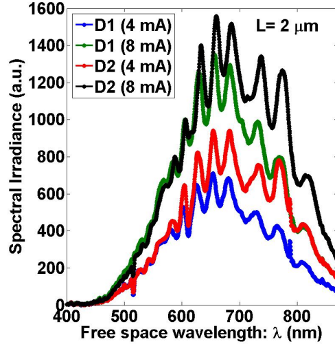
Fig. 11. Measured AM-EL spectral irradiance at 300 K for D1 and D2 at I_{AMLED}=4 \text{ mA} and 8 mA. The spectra are measured vertically using a 50 \mu\text{m} multi-mode optical fiber feeding an ADC-1000 USB spectrometer from Avantes.
