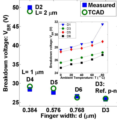
Fig. 10. TCAD simulated and measured V_{BR} for D2 to D6 at 300 K showing good agreement. The trend in V_{BR} is compliant with the one predicted by a 2-D analytical model [26]. (Inset): Measured V_{BR} at different ambient temperatures. Increasing V_{BR} with increasing temperature confirms the avalanche mechanism of breakdown.
