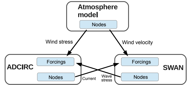
Figure 13. Schematic representation of the ADCIRC-SWAN coupling.
