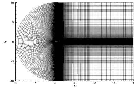
Fig. 1: NACA0014 computational mesh.
