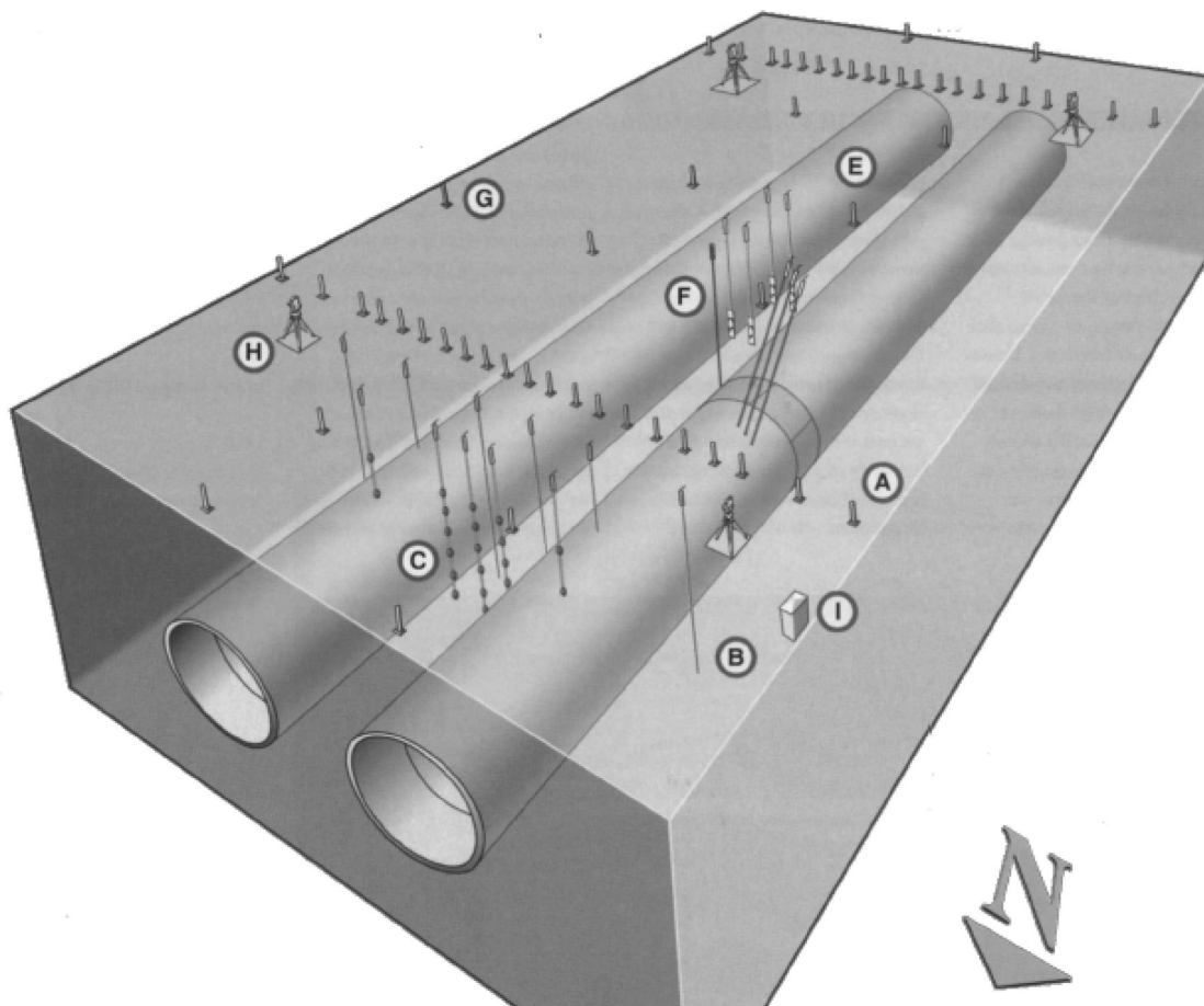
Fig. 3. Measuring field at Second Heinenoord Tunnel (reprinted from Broere 2001, with permission)
