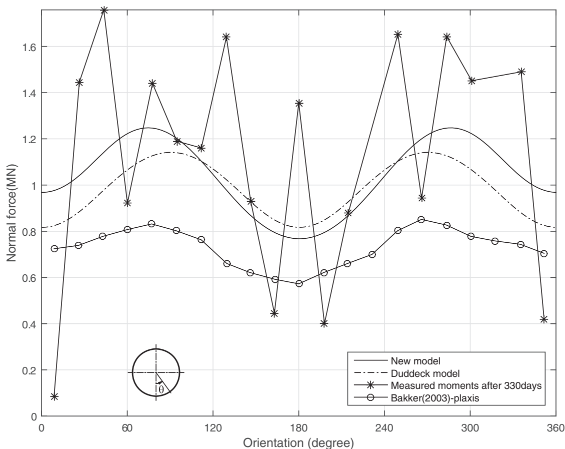
Fig. 6. Validation of normal forces in Second Heineoord Tunnel
