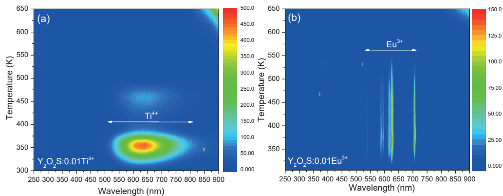
Figure 6.4. The thermoluminescence emission (TLEM) spectra of (a) \text{Y}_2\text{O}_2\text{S}:0.01\text{Ti}^{4+} and (b) \text{Y}_2\text{O}_2\text{S}:0.01\text{Eu}^{3+} . The heating rate is 1 K/s after and each sample has been exposed to an irradiation dose of 1.6 kGy from a ^{60}\text{Co} source.
