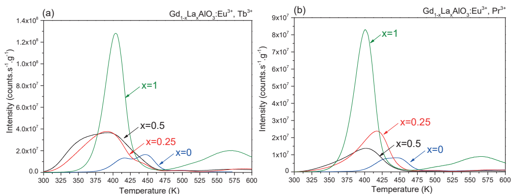
Figure S5.4. Unnormalized thermoluminescence glow curves of (a) \text{Gd}_{1-x}\text{La}_x\text{AlO}_3:0.01\text{Eu}^{3+}, 0.01\text{Tb}^{3+} and (b) \text{Gd}_{1-x}\text{La}_x\text{AlO}_3:0.01\text{Eu}^{3+}, 0.01\text{Pr}^{3+} . Both figures were measured by the RISØ TL-reader from 300 to 600 K with 1600 s irradiation by its \beta source and corrected by the mass. The heating rate was 1 K/s for all TL-recordings. A 600 nm bandpass filter (600FS40-50) was placed between the sample and PMT.
