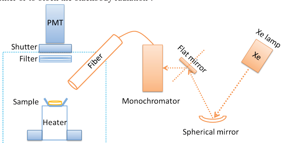
Figure 2.7. The schematic of the setup to measure the TLE spectra. The schematic is replotted from Ref.4.
