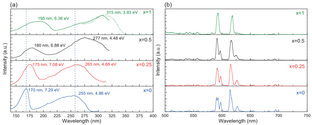
Figure 5.2. PLE (a) and PL spectra (b) of \text{Gd}_{1-x}\text{La}_x\text{AlO}_3:0.01\text{Eu}^{3+},0.01\text{Tb}^{3+} ( x=0, 0.25, 0.5 and 1). The excitation spectrum from 150 to 320 nm was measured by deuterium lamp excitation (solid line). The excitation spectrum from 250 nm to 400 nm was measured by Xe lamp excitation (dotted line). The excitation spectra were recorded at 592 nm emission and the emission spectra were excited at the charge transfer peak maxima. All measurements were performed at 10 K.
