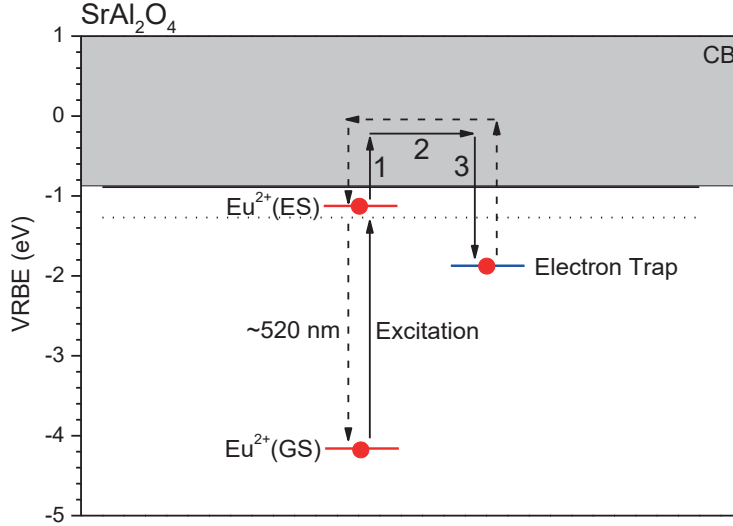
Figure 1.3. Illustration of the electron trapping (solid arrows) and detrapping (dashed arrows) processes in \text{SrAl}_2\text{O}_4:\text{Eu}^{2+}, \text{Dy}^{3+} . The filled circles stand for electrons.
