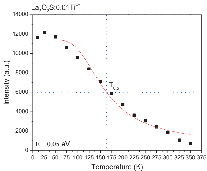
Figure S6.3. Thermal-quenching curve of \text{La}_2\text{O}_2\text{S:0.01Ti}^{4+} . The Black squares are measured and the red curve is fitted with Eq. 1.
