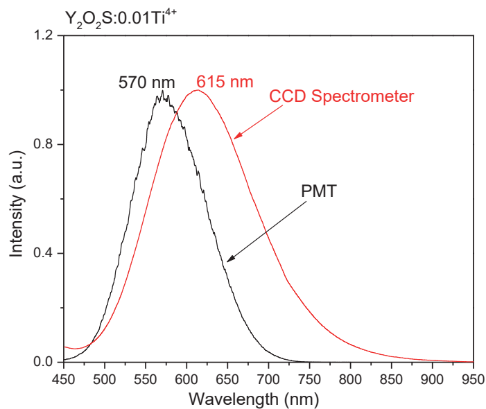
Figure S6.1. The comparison of the \text{Y}_2\text{O}_2\text{S:0.01Ti}^{4+} emission spectra measured by the PMT (EMI 9635QA) and CCD (QE65000). Both curves were excited by 365 nm UV radiation and recorded at room temperature (RT).
