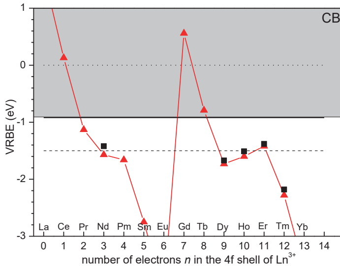
Figure 5.10. Comparison of the VRBE predicted by the VRBE diagram ( \blacktriangle ) and TL experiments ( \blacksquare ).
