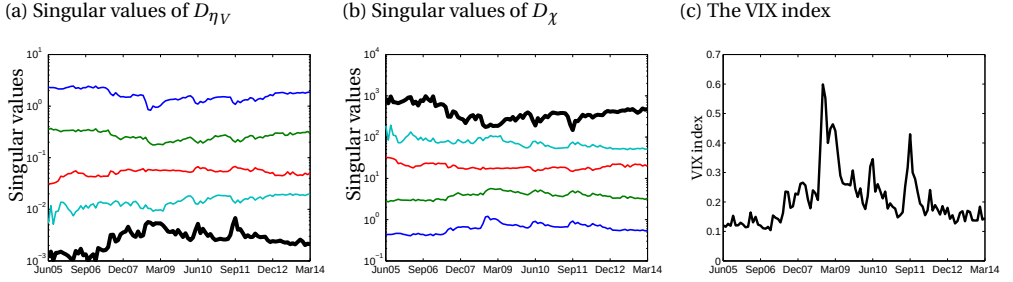
Figure 5.2: Numerical stability.
