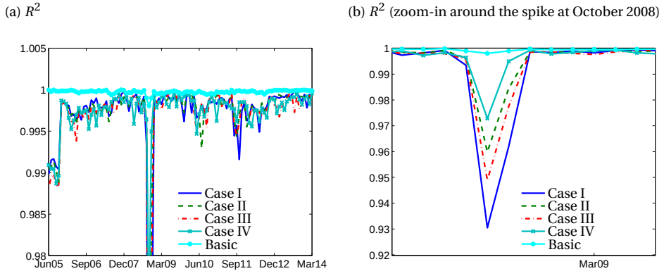
Figure 5.4: Quality-of-fit.
