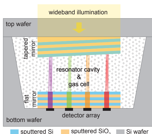
Figure 1. Side view of the gas-filled linear variable optical filter (LVOF), composed of a flat and a tapered mirror with a tapered resonator cavity in-between.
