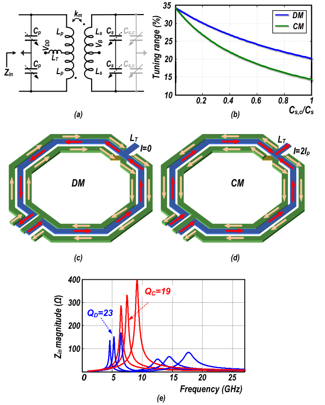
Fig. 2. (a) a transformer-based tank; (b) limited DM and CM TR due C_s, c ; 1:2 turn transformer; (c) DM excitation; (d) CM excitation; and (e) tank's input impedance.
