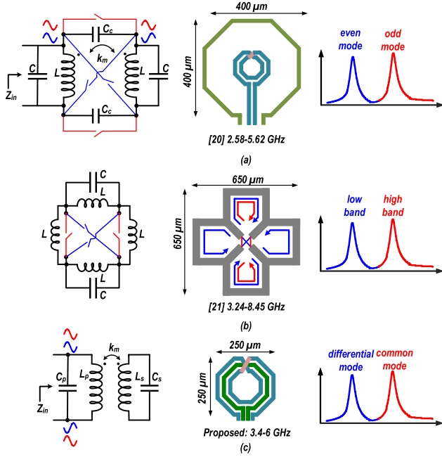
Fig. 1. LC-tanks for wide tuning range: (a) resonant mode switching technique [20]; (b) band switching technique [21]; (c) proposed technique.
