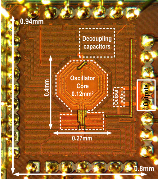
Fig. 10. Chip micrograph.
