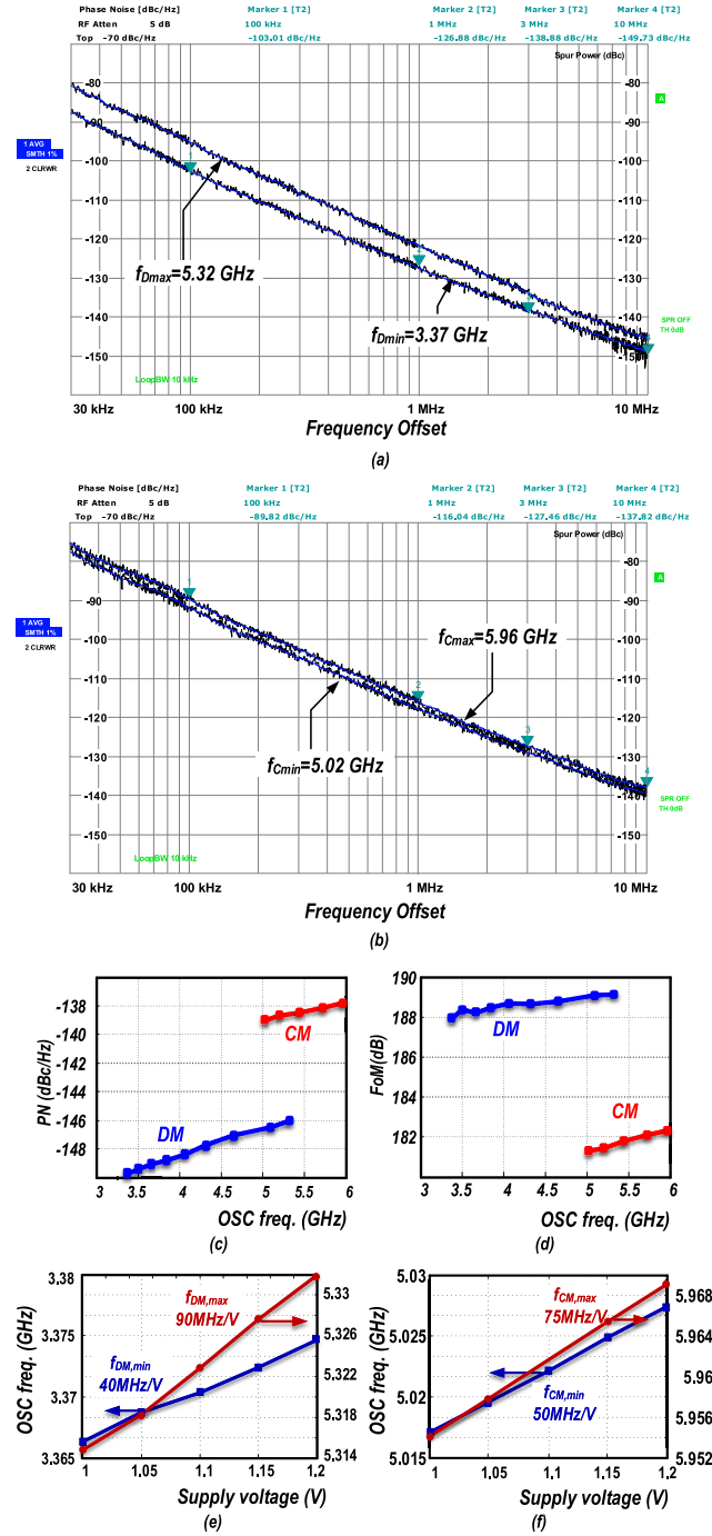
Fig. 12. Measurements: (a) PN at f_{DM,max} , f_{DM,min} , and (b) f_{CM,max} and f_{CM,min} ; (c) PN and (d) FoM at 10MHz offset across TR. Frequency pushing due to supply voltage variation in (e) DM, and (f) CM oscillators.
