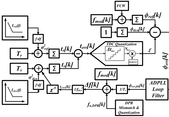
Fig. 10. Time-domain model of ILFM with impairments.
