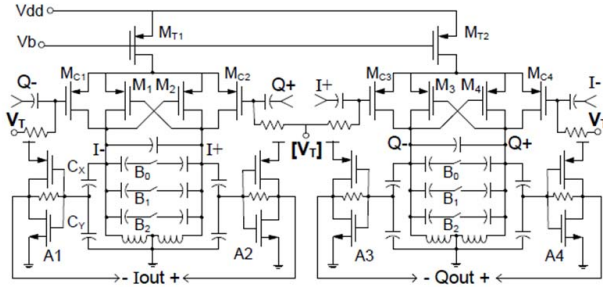
Fig. 5. QVCO with frequency tuning by varying coupling strength [10].
