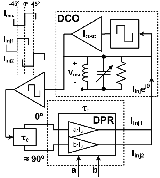
Fig. 7. Block diagram of the wideband frequency modulator through self-injection locking [12].
