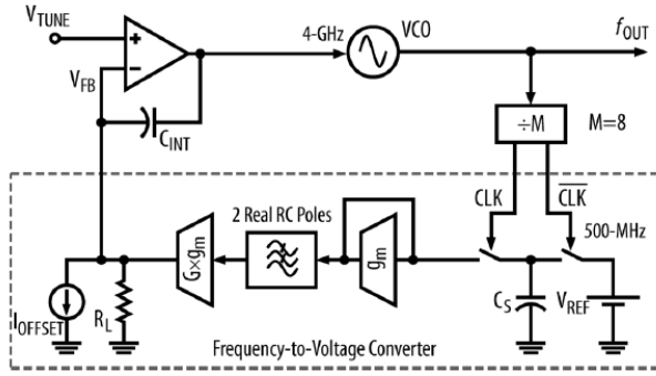
Fig. 4. Wideband frequency modulator using frequency-to-voltage converter in negative feedback loop.
