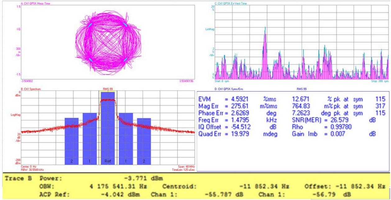
Fig. 12. VSA simulation result with 1% mismatch in DPR array.
