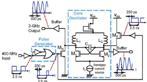
Fig. 6. Injection-locked transmitter for narrowband FM [11].
