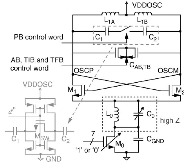
Fig. 1. DCO with capacitive tuning [4].
