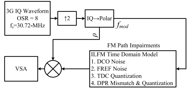
Fig. 9. System test bench of DFC employing ILFM.
