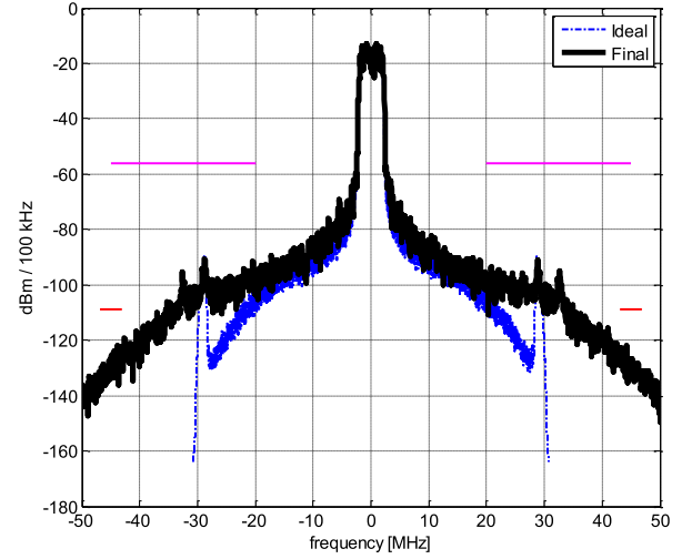
Fig. 11. Wideband spectrum simulated with 2% mismatch in DPR array.
