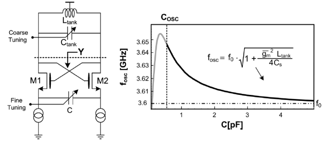
Fig. 2. High-resolution DCO using capacitive degeneration [7]. Left: circuit diagram. Right: DCO frequency versus tuning capacitance.
