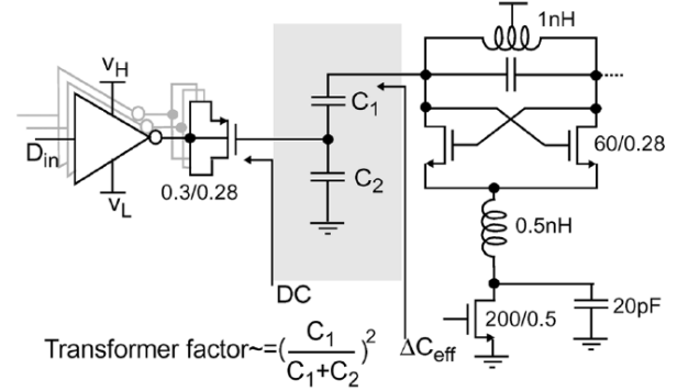
Fig. 3. DCO with capacitive transformer [8].
