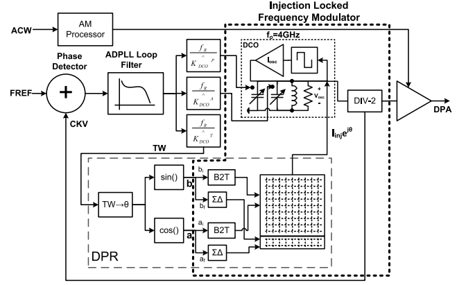
Fig. 8. Block diagram of complete TX system employing ILFM.
