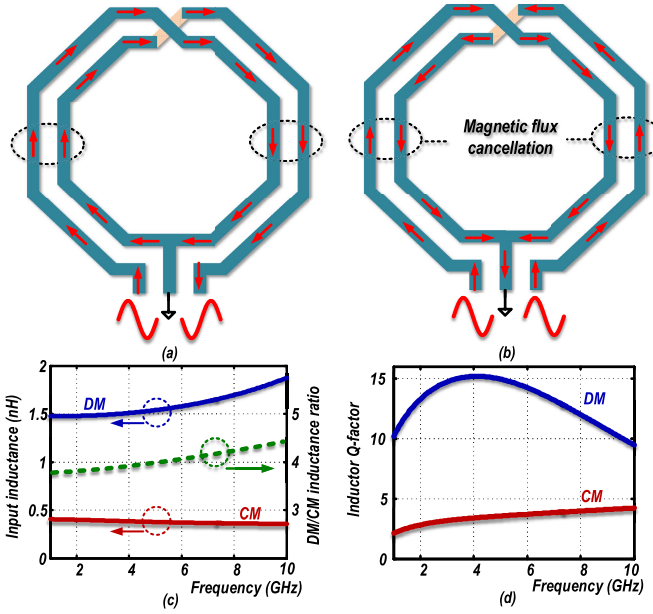
Fig. 9. Two-turn “F 2 ” inductor in (a) DM excitation, (b) CM excitation, (c) F 2 DM and CM inductances and their ratio, and (d) Q_{DM} and Q_{CM} .
