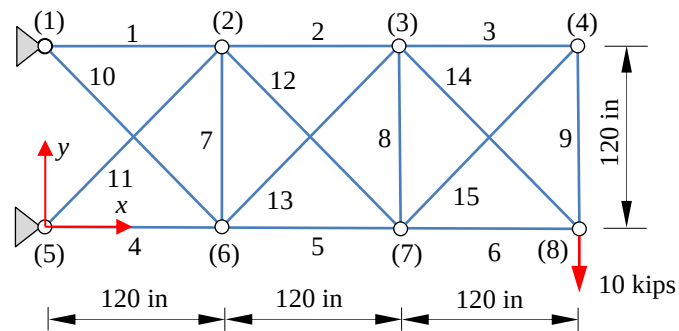
Fig. 6. The 15-bar planar truss.
