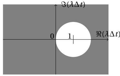
Figure 3.6: Stability region: Stable outside of the circle
