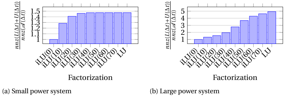
Figure 7.2: Normalized number of non-zeros in the incomplete factorization of \mathcal{A}(\Delta t) for various levels of fill-in, and the LU factorization of \mathcal{A}(\Delta t) for the small (a) and large (b) power systems.
