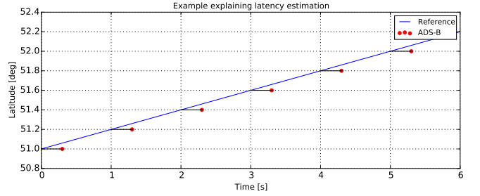
Fig. 1. Example explaining latency estimation
