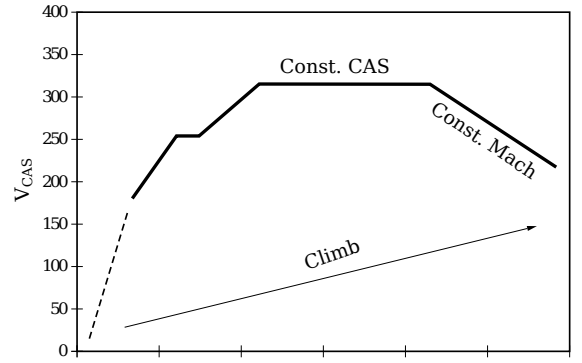
Fig. 3. Standard climb profile
