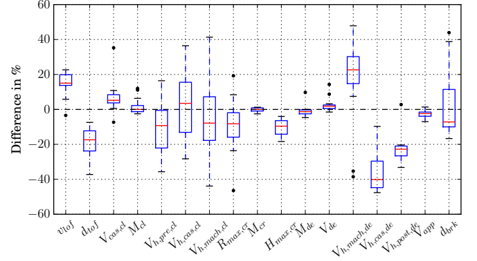
Fig. 17. Comparison with Eurocontrol Aircraft Performance Database
