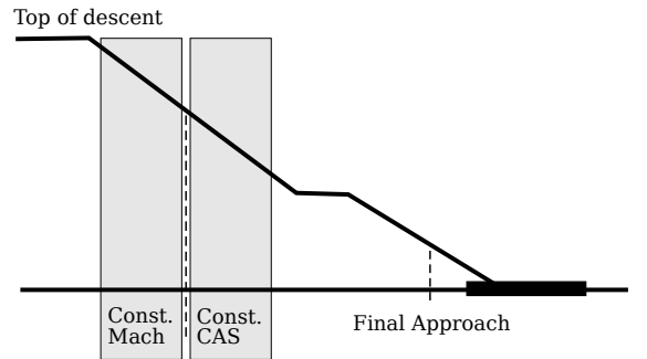
Fig. 7. Standard descent profile
