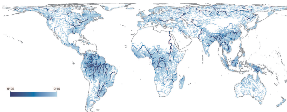
Figure A.1: Average river discharge in 2000 ( km^3/yr ), using data from [54].
