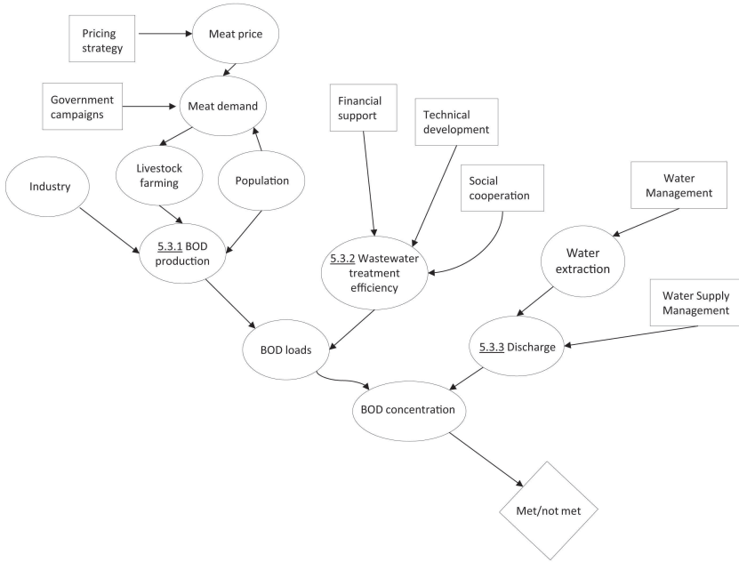
Figure 5.1: Influence diagram model for improving organic river pollution. Oval nodes represent variables, rectangular nodes indicate decisions and the diamond node represents the outcome or utility, in this case the extent to which BOD concentration targets are met.
