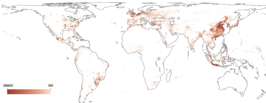
Global distribution of intensive poultry production systems in year 2000 ( \text{stock}/\text{km}^2 )
