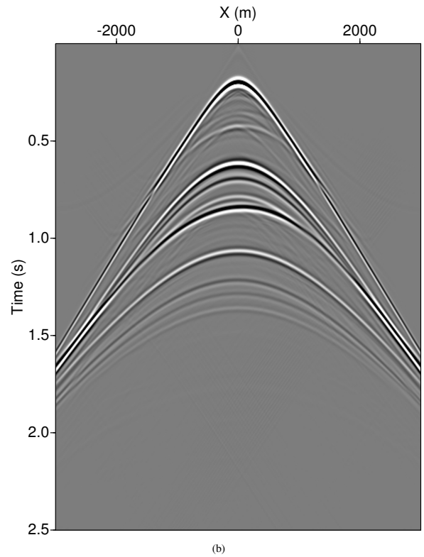
Figure 4: Retrieved primaries after one (a) and 20 (b) iterations.
