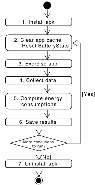
Fig. 1: PETRA: workflow
