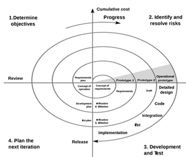
FIGURE 43 A SPIRAL MODEL OF SOFTWARE DEVELOPMENT AND ENHANCEMENT, ADAPTED FROM BOEHM (BOEHM, 1986)
