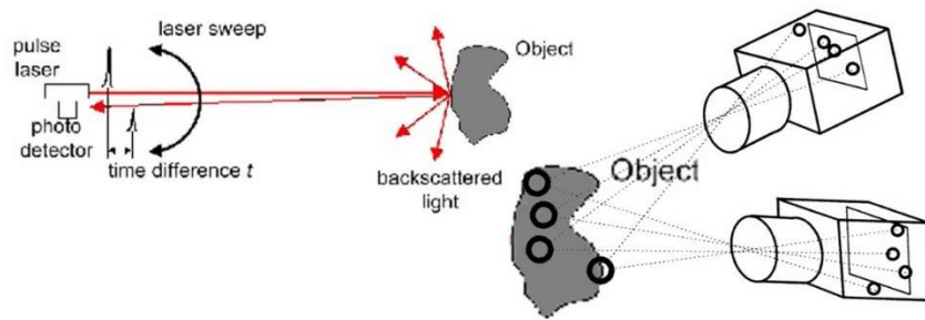
FIGURE 24 TWO METHODS TO EXTRACT 2,5D SPATIAL KNOWLEDGE
