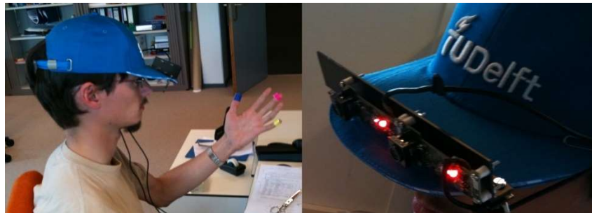
FIGURE 54 COLOR CODED HAND TRACKING SUBSYSTEM
