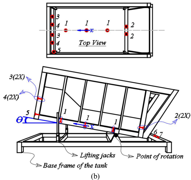
Fig. 1. (a) The liquefaction tank (b) Overview of instrumentation in the liquefaction tank.
