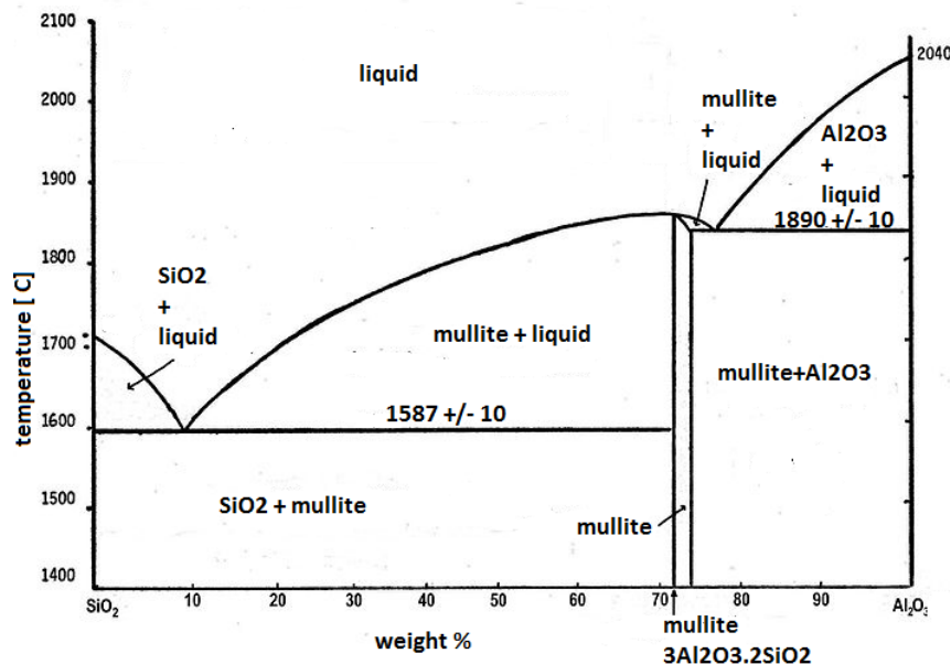
Figure 2.6: Phase diagram for the system \text{Al}_2\text{O}_3 - \text{SiO}_2 [2.25]
