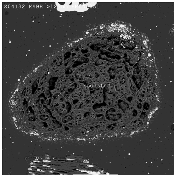
Figure 4:10: SEM photograph of organic coarse particle in coal fly ash, reference of co-combustion of paper sludge (PSE) (back-scattered plot). Particle consisting of char with spherical sub particles mainly at the surface. Incomplete char burn-out whereby the included minerals were melted during combustion and formed a kind of a layer on the surface.
