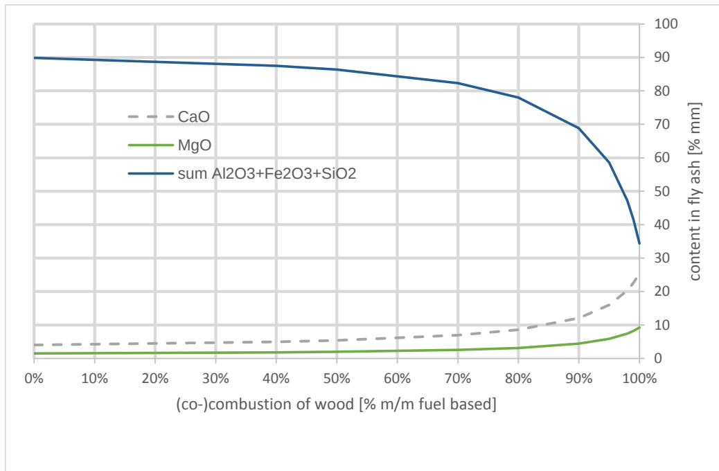
Figure 6:5: Calculated concentration of CaO, MgO and sum of, \text{Al}_2\text{O}_3 , \text{SiO}_2 and \text{Fe}_2\text{O}_3 equivalent in fly ash as function of the share of wood in the fuel.
