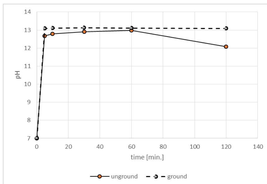
Figure 5:3: Development of pH of water after addition of ground or unground wood fly ash WD100-1 (10 grams of fly ash in 100 ml demineralized water)
