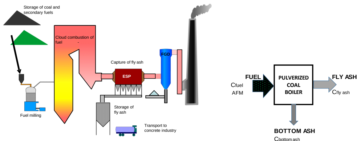
Figure 6:1: Principle of coal fired power plant (left) and simplified mass balance (right).
