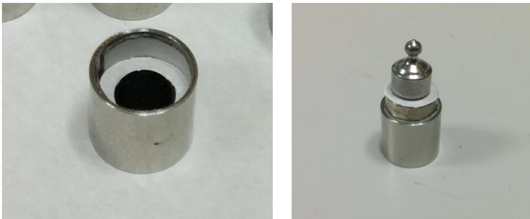
a. b. Figure 6. a. A bitumen sample in a storage container, with the silicon paper fixing the contact area showing on top b. An assembled test specimen with a small weight placed on top.
