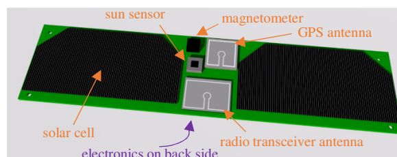
Figure 9. Artist impression of an advanced outer panel, suitable for a 3p PocketQube.
