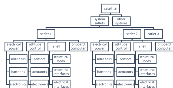
Figure 2. Example physical breakdown of a cellularized satellite using ‘system satlets’
