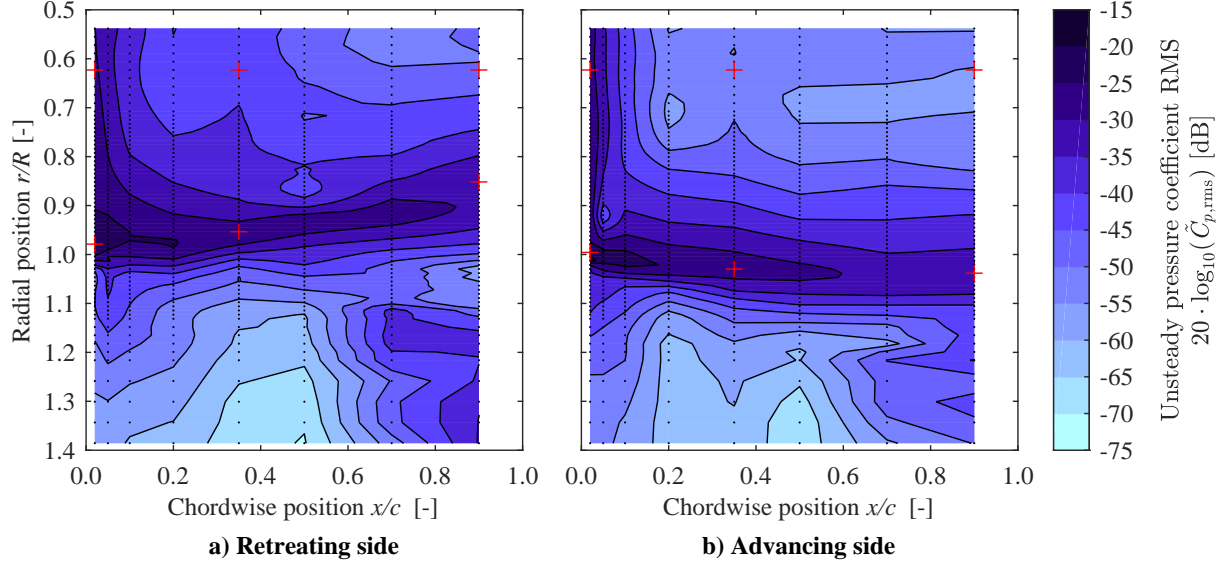
Figure 8. Contours of the rms of the pressure fluctuations over the pylon surface in the baseline configuration, expressed in logarithmic scale relative to freestream dynamic pressure.
