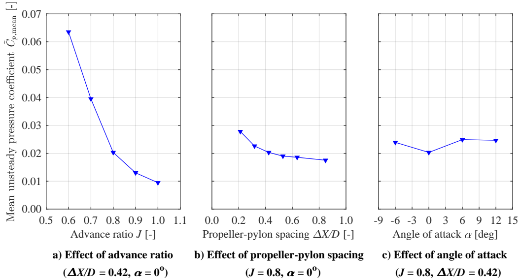
Figure 12. Average unsteady pressure coefficient versus advance ratio, propeller-ptyon spacing, and angle of attack.
