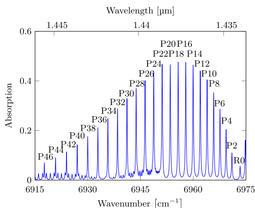
FIG. 4. Nomenclature of the investigated CO 2 absorption lines in the 3 ν 3 band 41 as labelled in HITRAN. The shown absorption profile corresponds to 1.5 m of propagation through pure CO 2 at the pressure of 1 atm and a temperature of 296 K.
