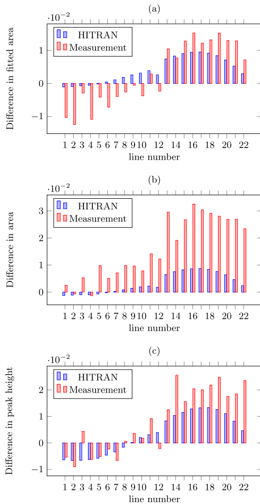
FIG. 7. Changes in absorption for the different investigated absorption lines when increasing the temperature by \approx 10 K (from 26.9 °C to 36.7 °C). The beam propagated through 1.5 m of pure CO 2 at a pressure of 1 atm. The reference image was taken by flushing the cell with N 2 . (a) Comparison of the area under the curve when fitting a multi-line Lorentzian profile. The measured temperature would be interpreted to be 5 K higher than the read-out from HITRAN, with an estimated uncertainty of 3 K. (b) Comparison when the lines are simply integrated without assuming any line shape. In (c) only the peak height was compared. The measurement (shown in red) generally shows a stronger reaction to the temperature changes than HITRAN data (blue).
