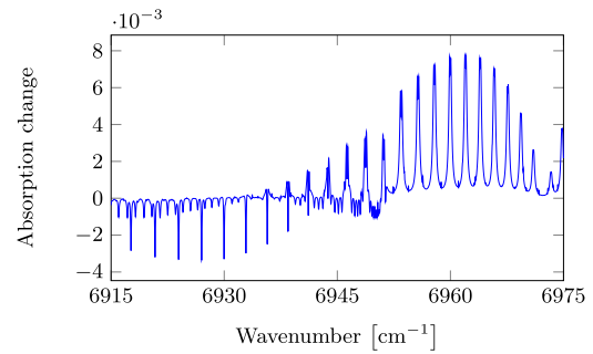
FIG. 5. Expected change when increasing the temperature of pure CO 2 by 5 K. The plot shows the absolute difference in absorption [A(T = 296 \text{ K}) - A(T = 301 \text{ K})] for propagation through 1.5 m pure CO 2 at a pressure of 1 atm. The strength of the corresponding absorption lines is shown in Fig. 4.
