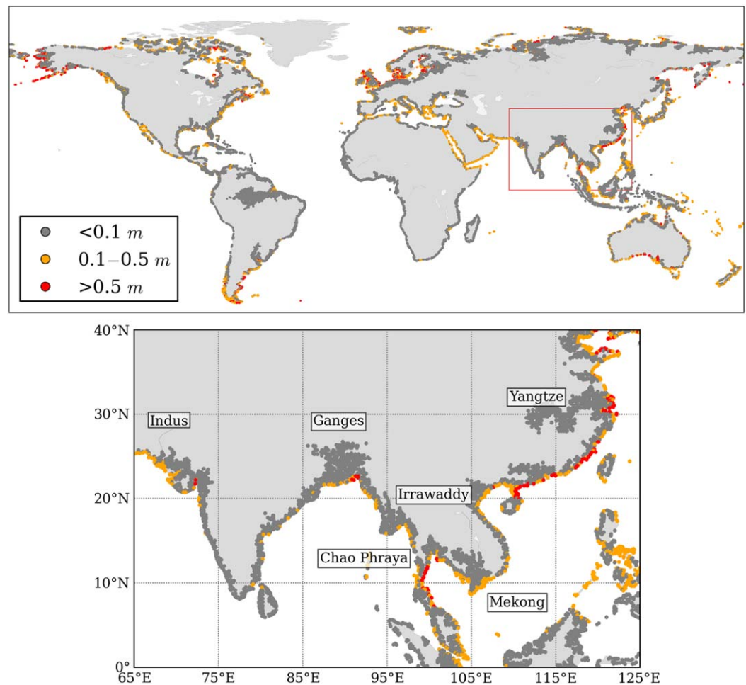
Figure 1. Difference in annual maxima of water surface elevation (m) for the year 2005 between simulations with and without GTSR at a global-scale (top figure) and a continental-scale (Asian region, bottom figure). The magnified domain shown in the bottom figure is indicated as a red rectangle in the top figure.
