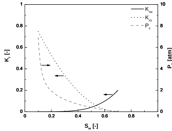
Figure 4.2 The relative permeability and capillary-pressure functions for matrix blocks in all the cases in this study.
