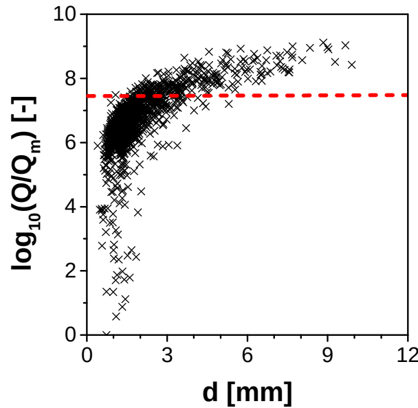
Figure 2.22 Q of each fracture normalized by the minimum value of Q of all the fractures in log-10 space plotted against aperture: aperture is proportional to fracture length. Results of one realization shown. The red dashed line indicates the value of Q below which the fractures are eliminated in this case.
