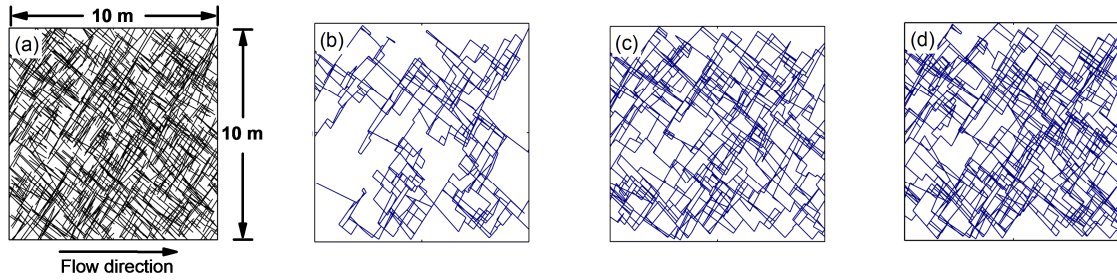
Figure 2.4 (a) One realization of the fracture network examined in this study. The size of the fractured region is 10 \text{ m} \times 10 \text{ m} \times 0.01 \text{ m} . The left and right boundaries are each at fixed hydraulic head; the difference in hydraulic head is 1 m. Water flows from left to right; the top and bottom edges are no-flow boundaries. (b) Dominant sub-network for one realization with a power-law aperture distribution with \alpha = 1.001 . (c) Dominant sub-network for one realization with a power-law aperture distribution with \alpha = 2 . (d) Dominant sub-network for one realization with a power-law aperture distribution with \alpha = 6 .
