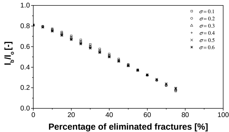
Figure 2.15 Length of sub-network backbone ( l_b ) normalized by the total length of the original fracture network ( l_o ) plotted against the percentage of eliminated fractures, for the cases of log-normal aperture distributions with the same log-mean value but different log-standard deviations ( \sigma ) from 0.1 to 0.6. Average trend curve for 100 realizations shown for each value of \sigma .
