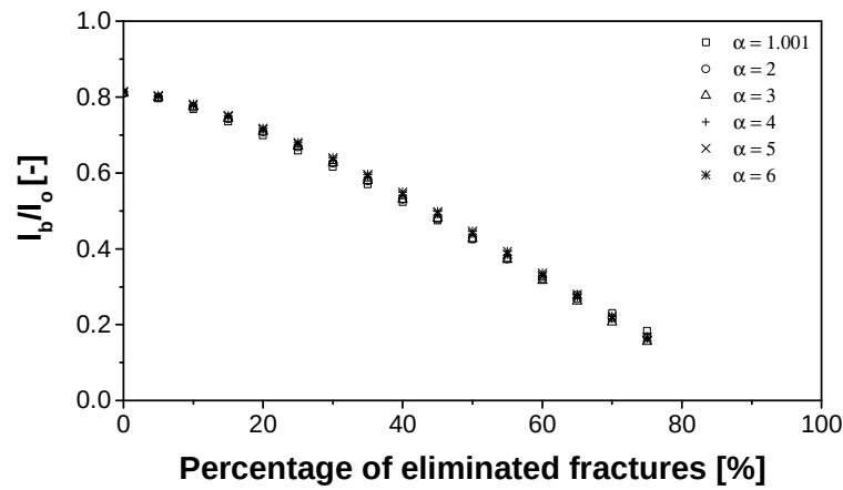
Figure 2.5 Length of the backbone of the truncated fracture network ( l_b ) normalized by the total length of the original fracture network ( l_o ) plotted against percentage of eliminated fractures, for power-law aperture distributions with exponent \alpha = 1.001 to 6. Average trend curve for 100 realizations shown for each value of \alpha .
