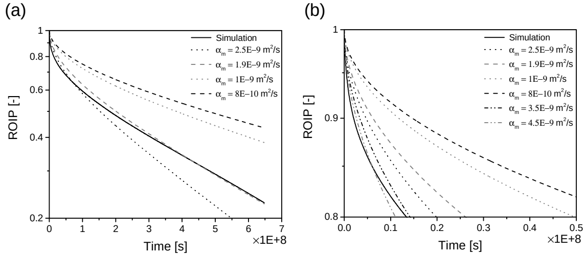
Figure A.3 Fraction of remaining oil in place (ROIP) for a 2D recovery process calculated numerically (solid line) and with constant coefficient \alpha_m for different values of \alpha_m . (a) long time scale, during which most oil is recovered. (b) Short times.
